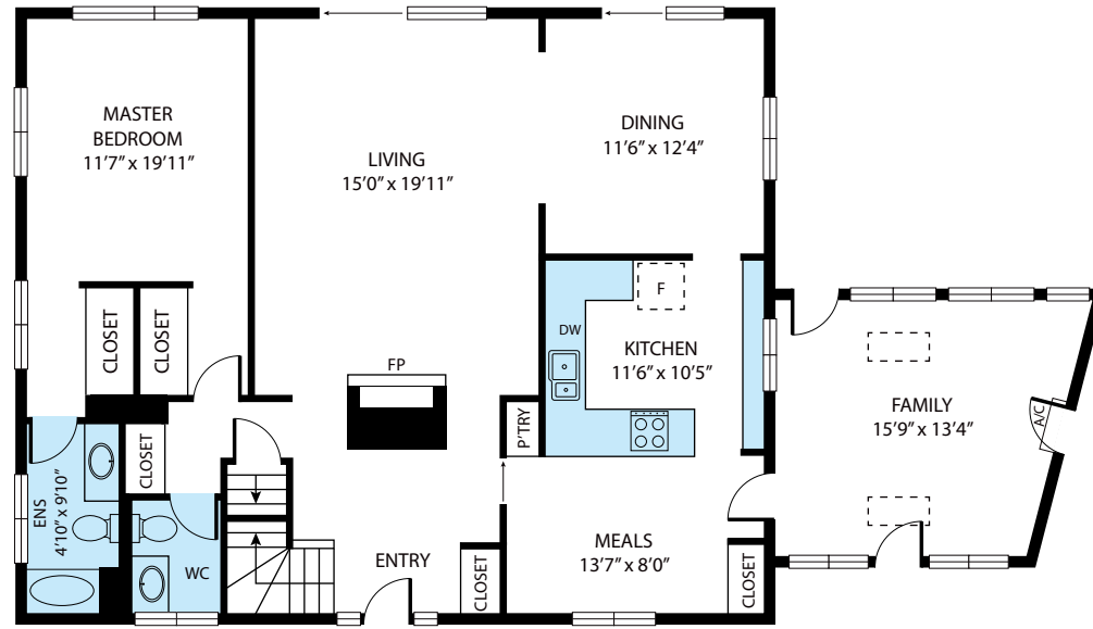
FIRST FLOOR
