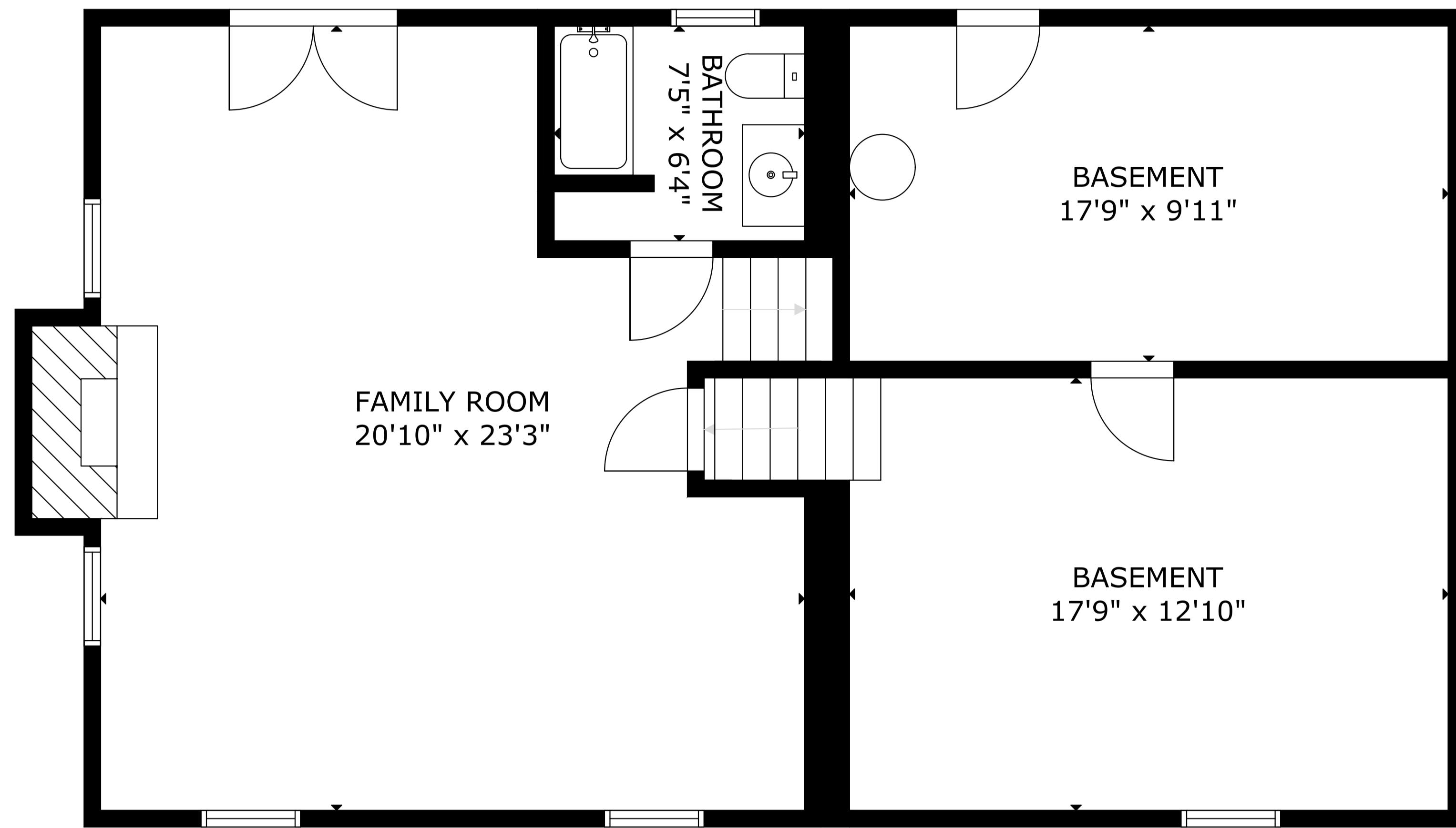
LOWER FLOOR
