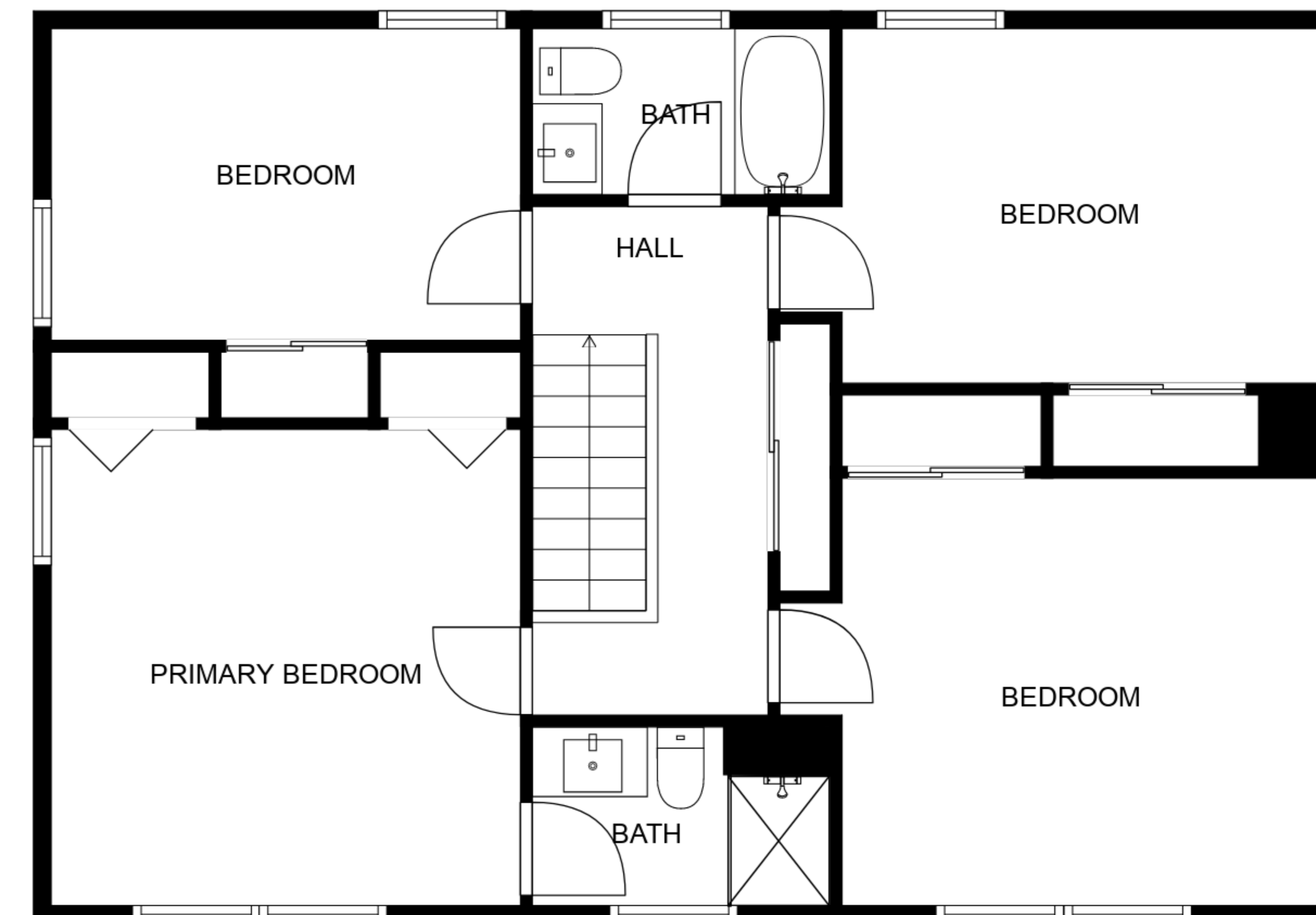
FLOOR 3
