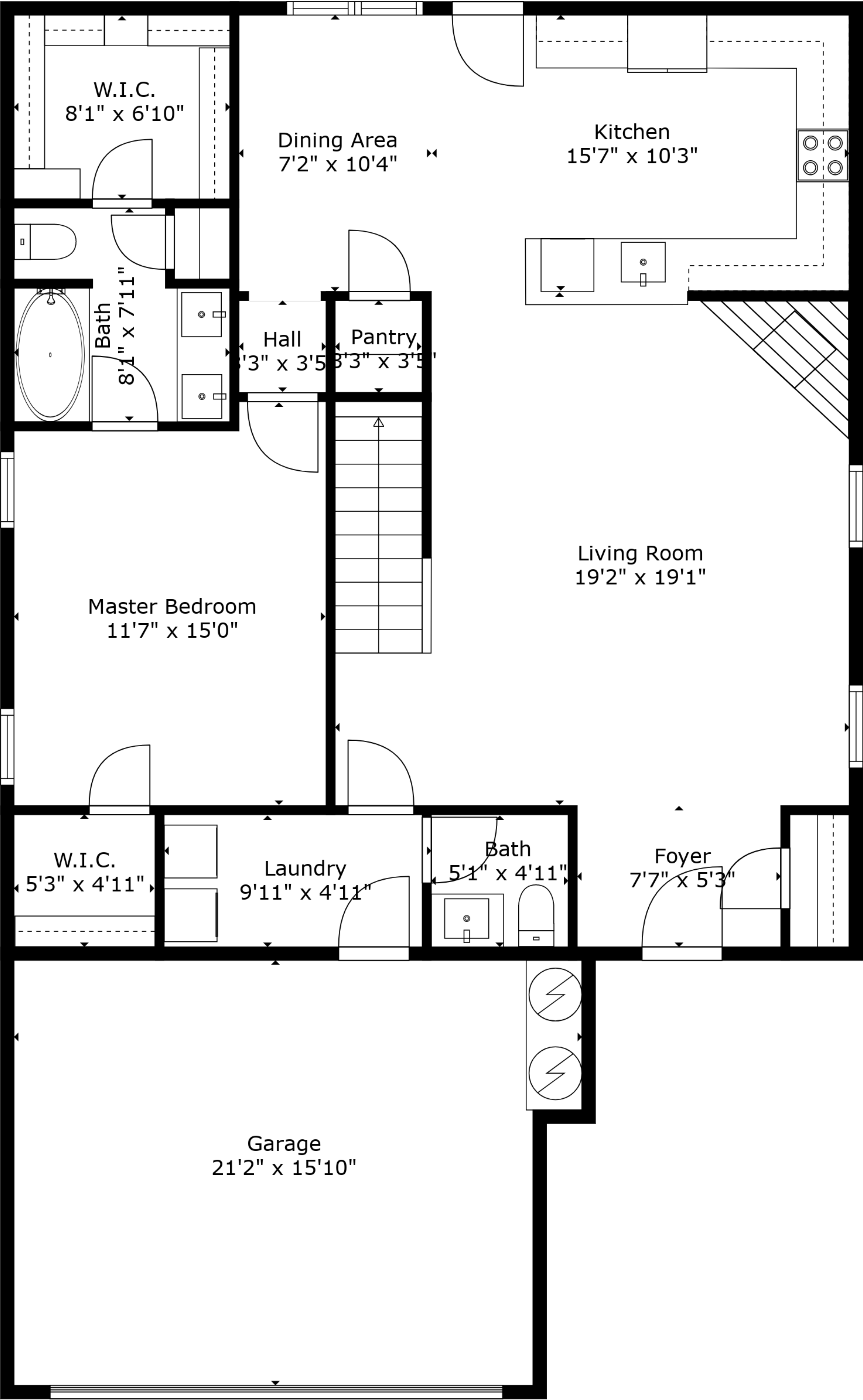
Floor 1
