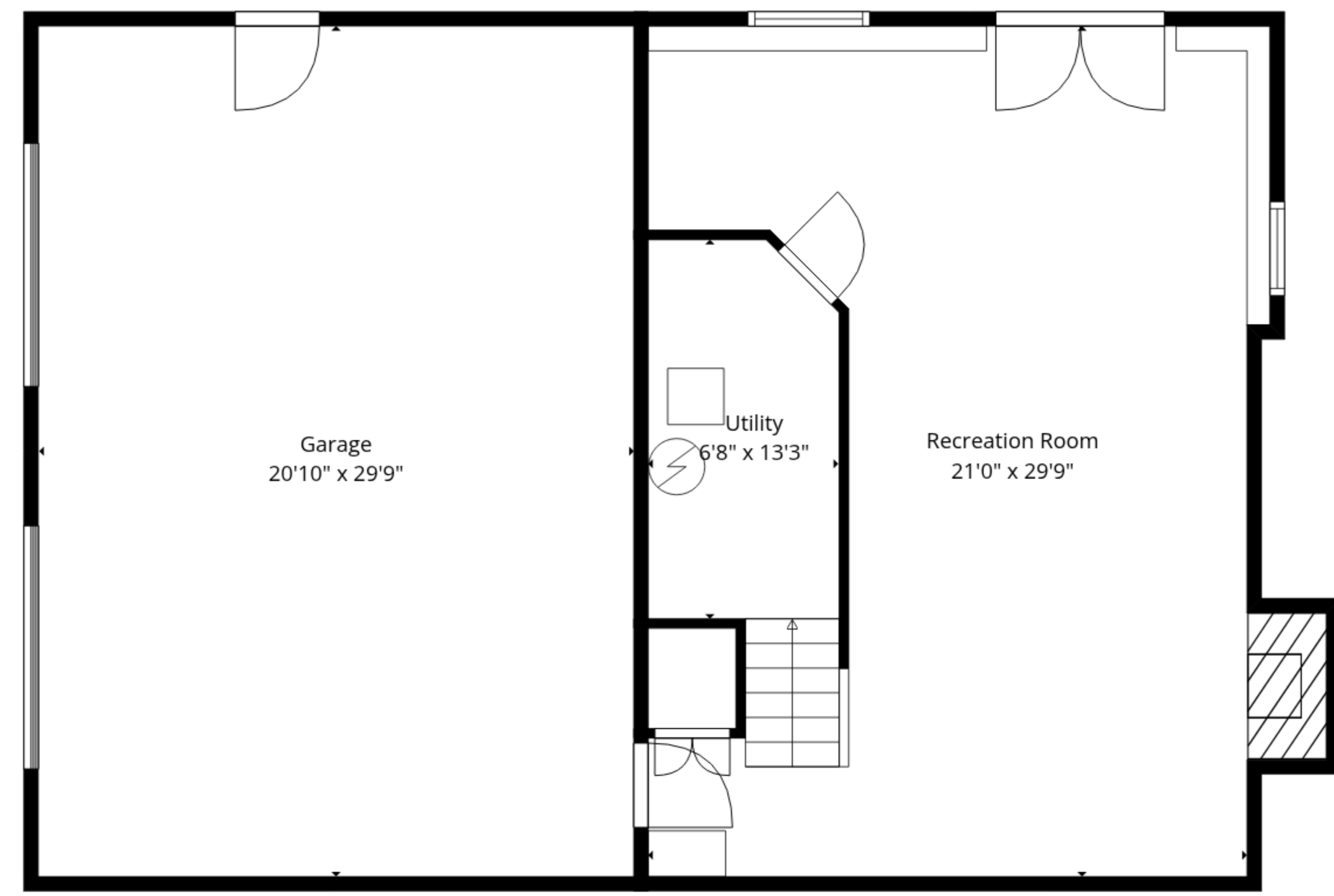
Basement
