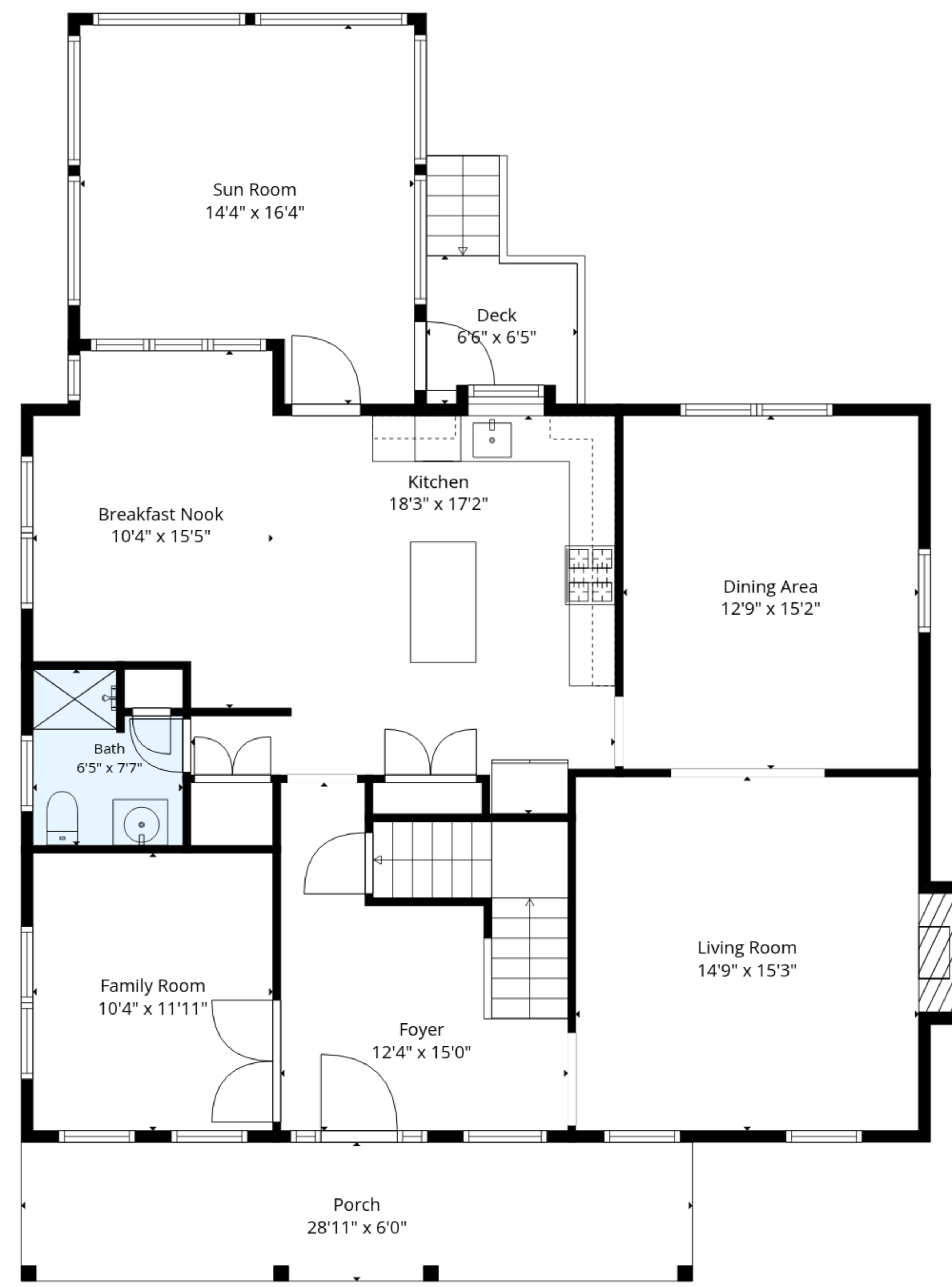
1st Floor
