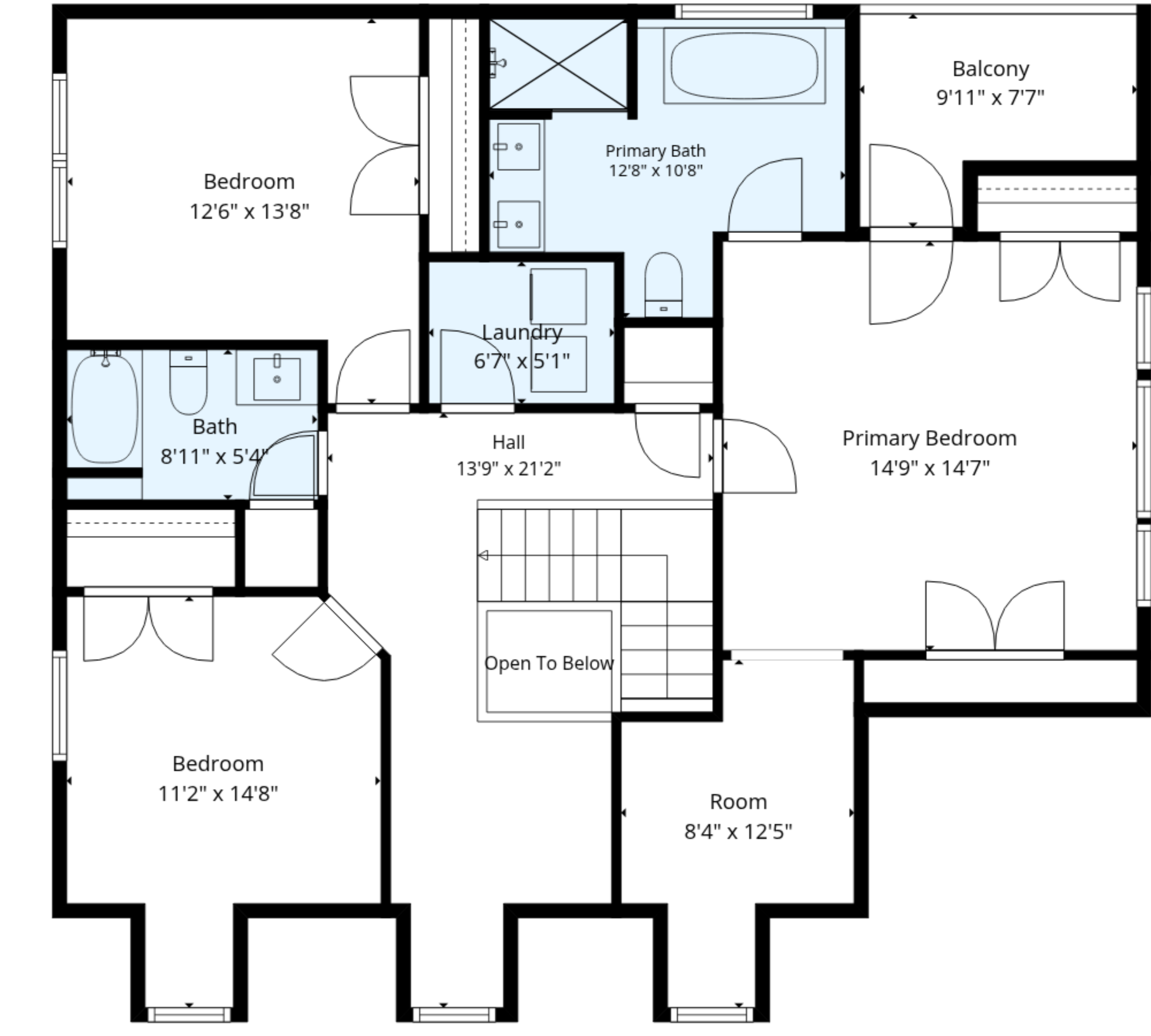
2nd Floor
