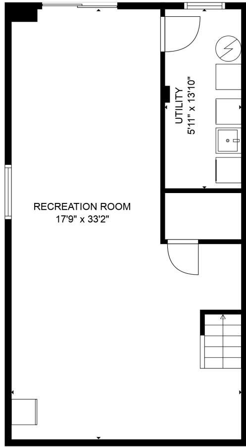
FLOOR 1
