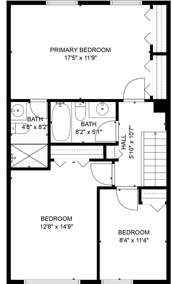
FLOOR 3
