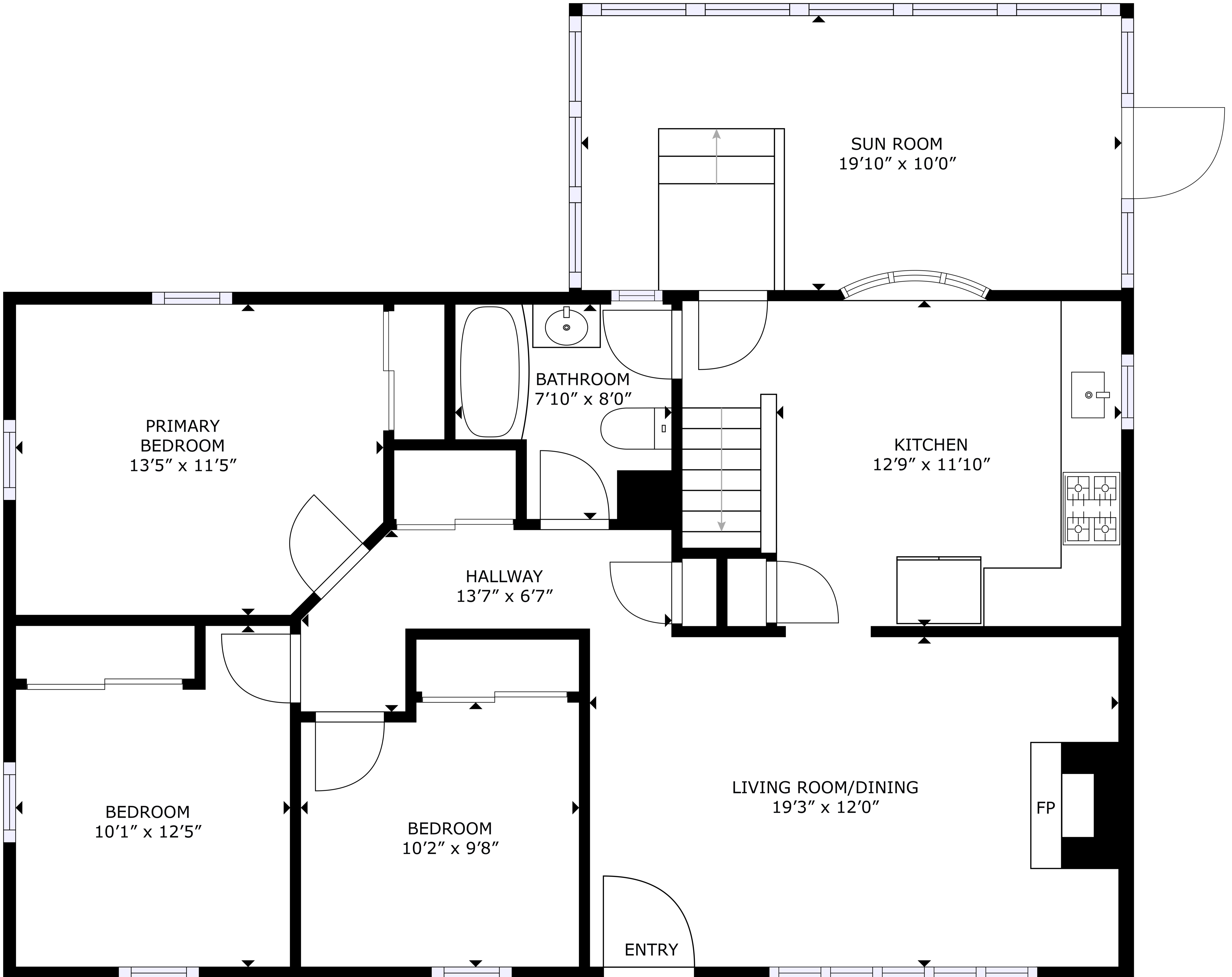
FLOOR PLAN
