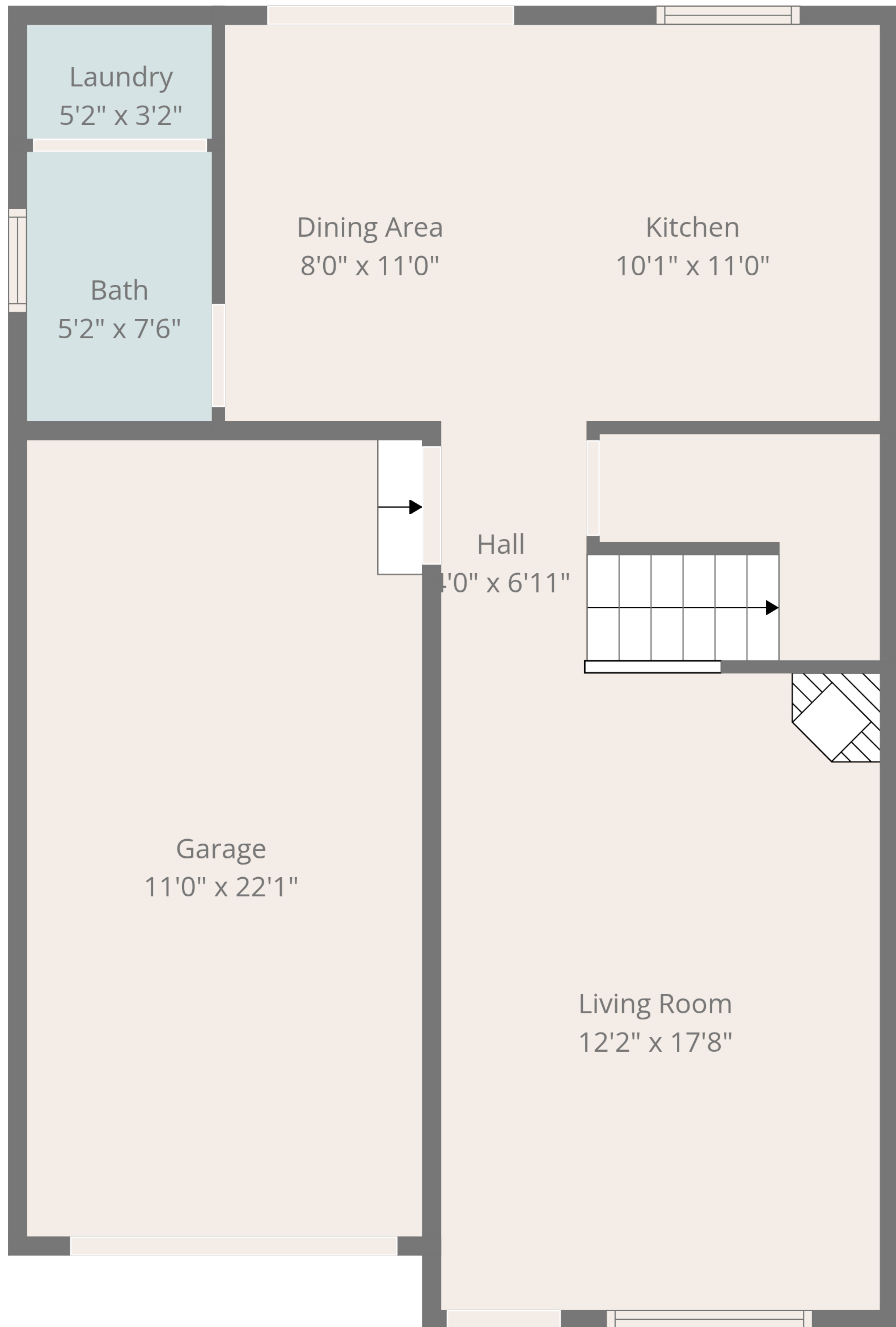
1st Floor
