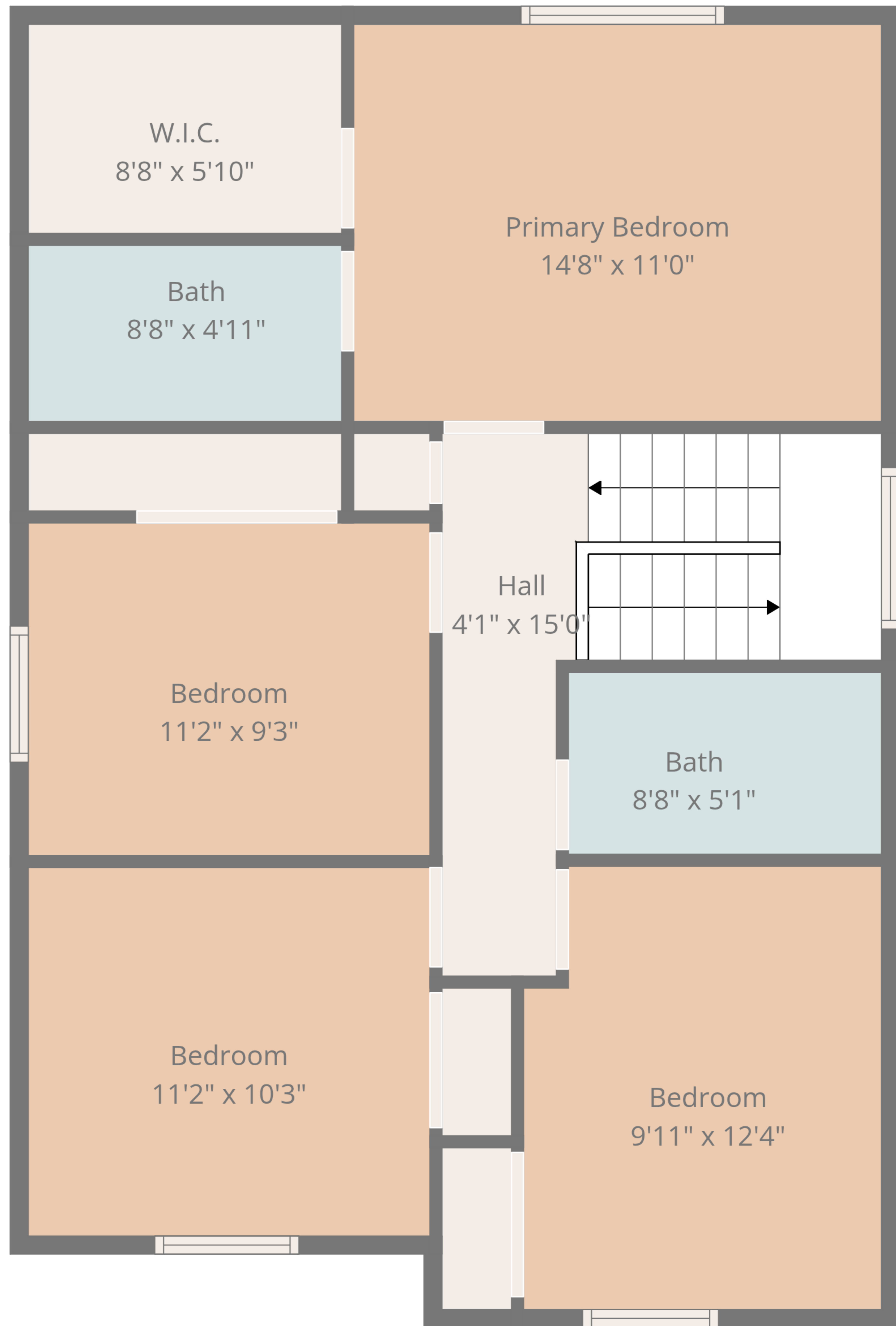
2nd Floor
