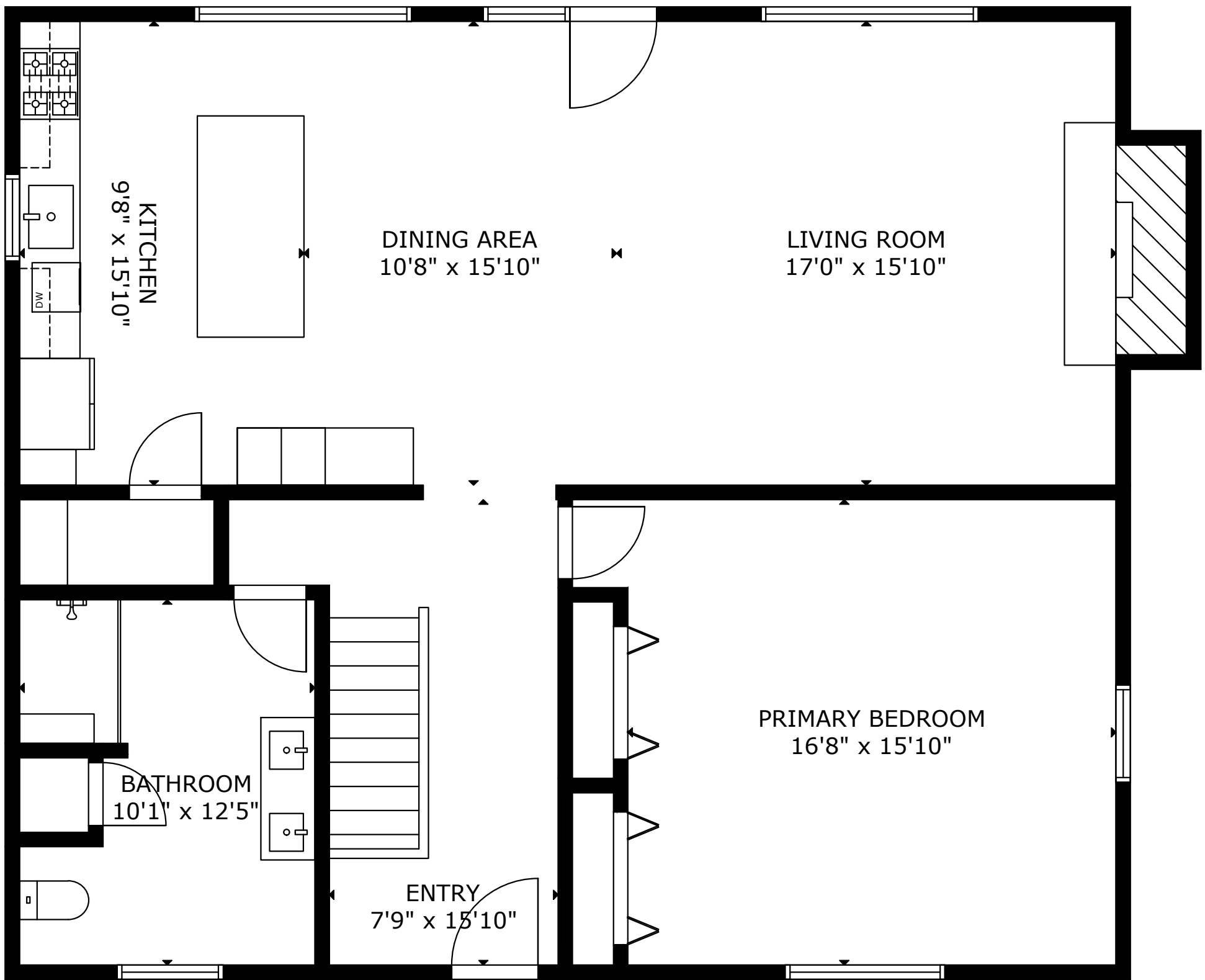
MAIN FLOOR
