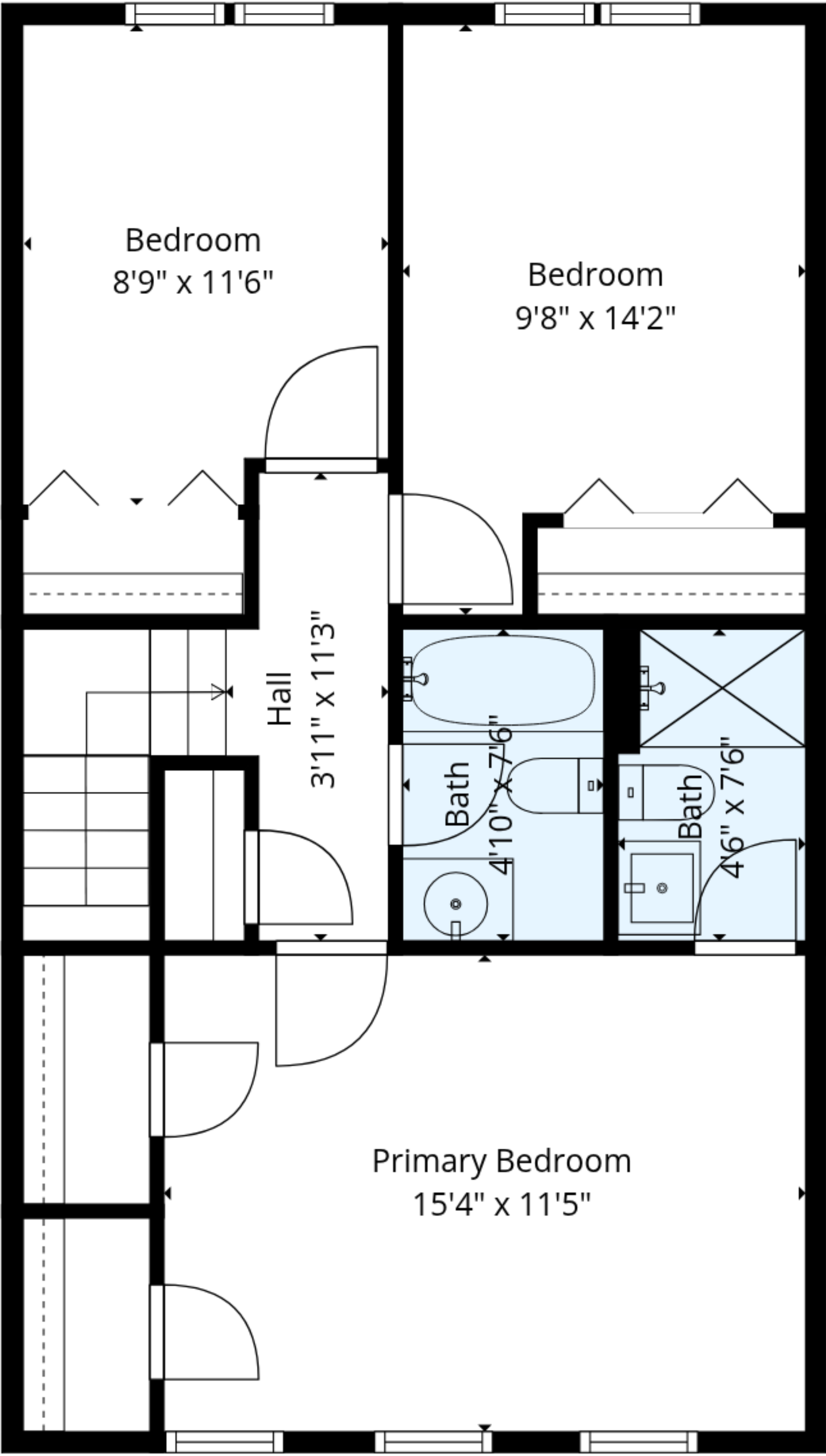
Floor 3
