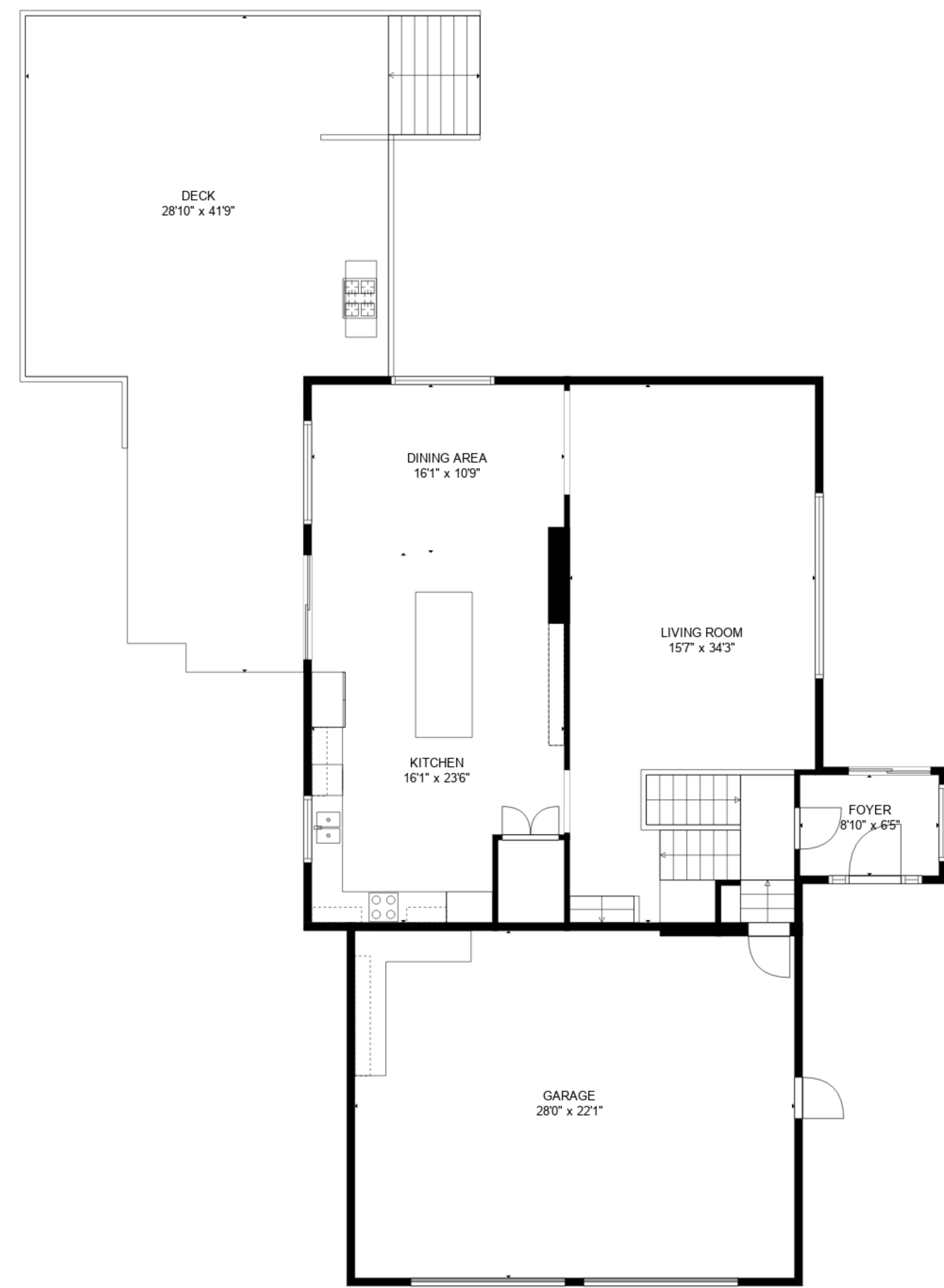
FLOOR 2
