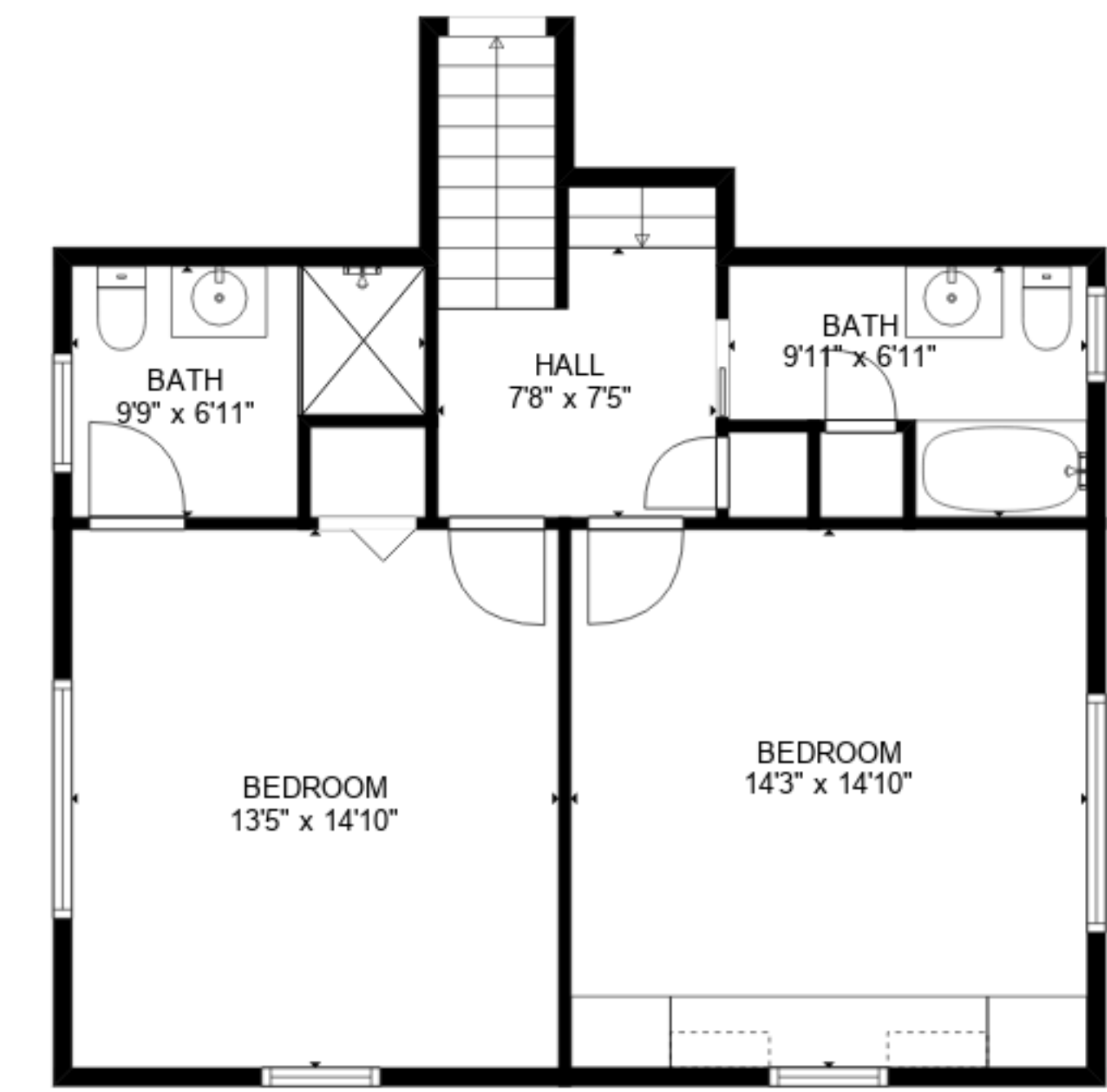
FLOOR 3
