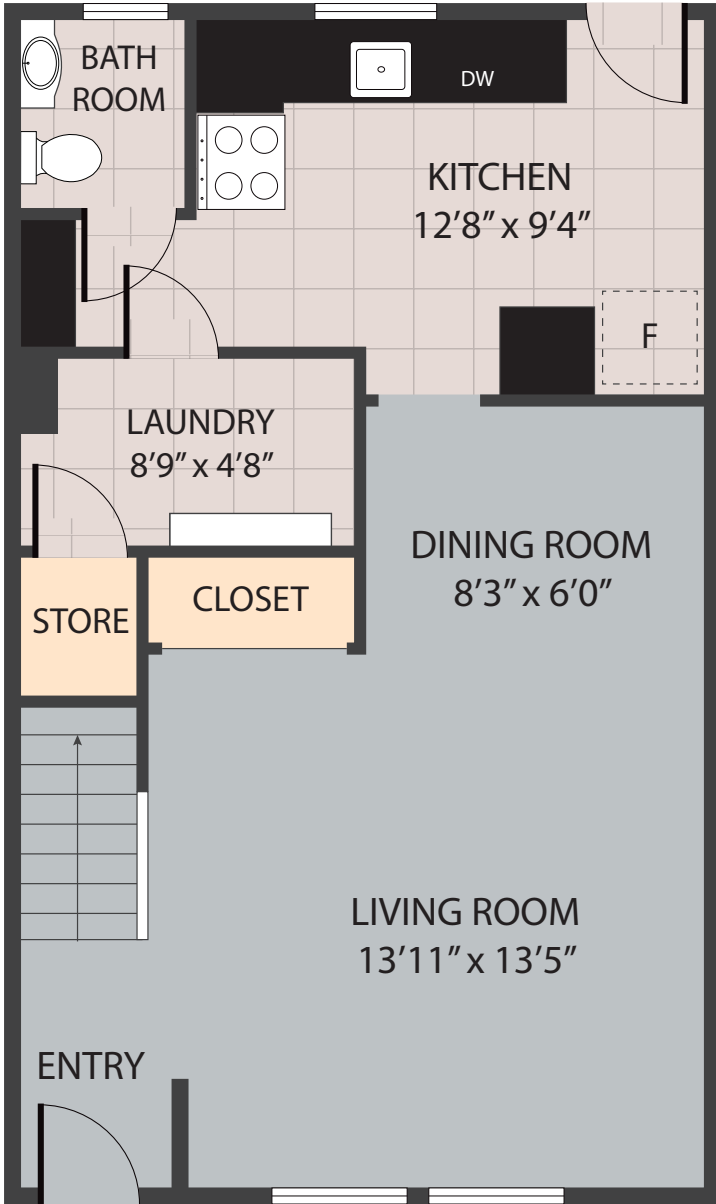
FIRST FLOOR
