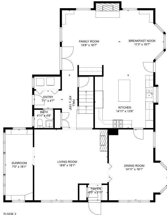
FLOOR 2
