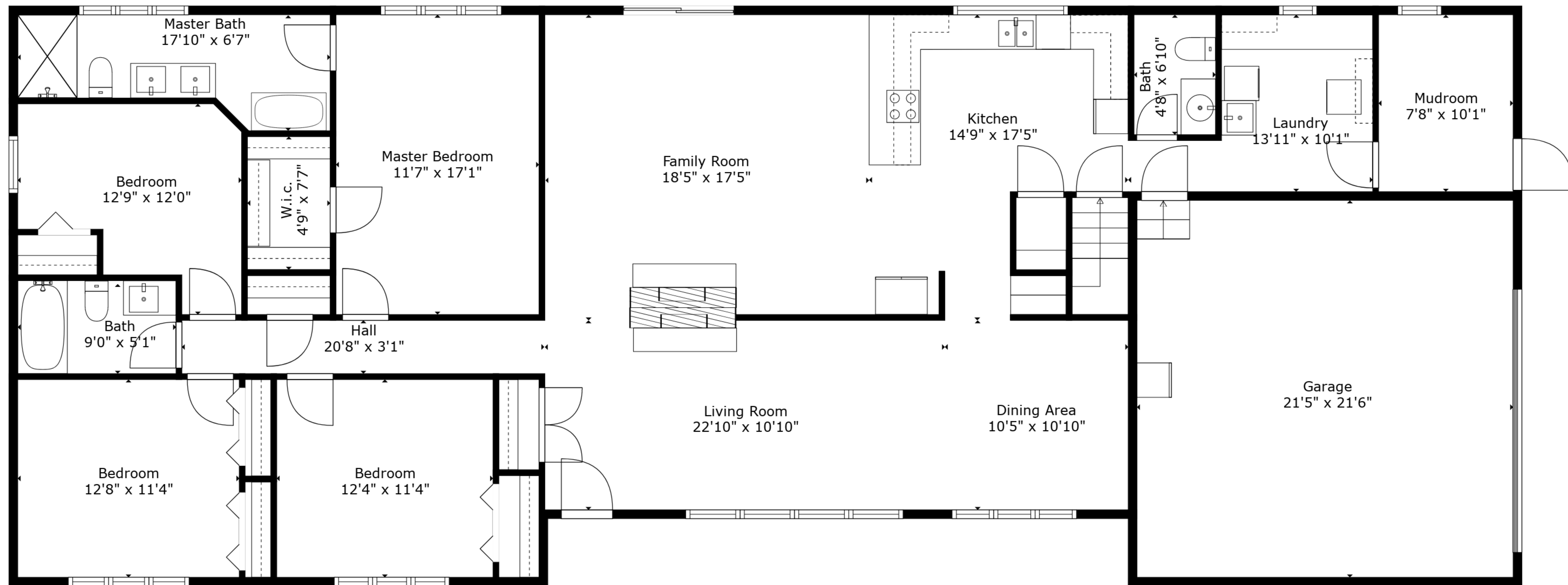
Floor 2
