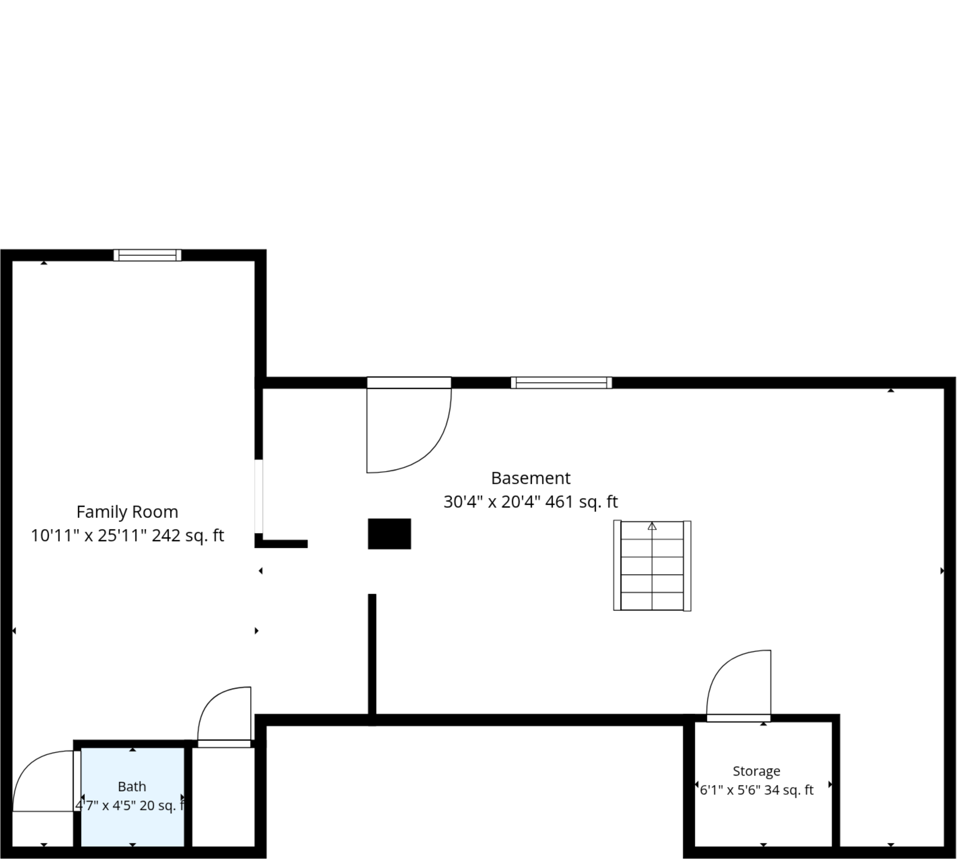
Basement
