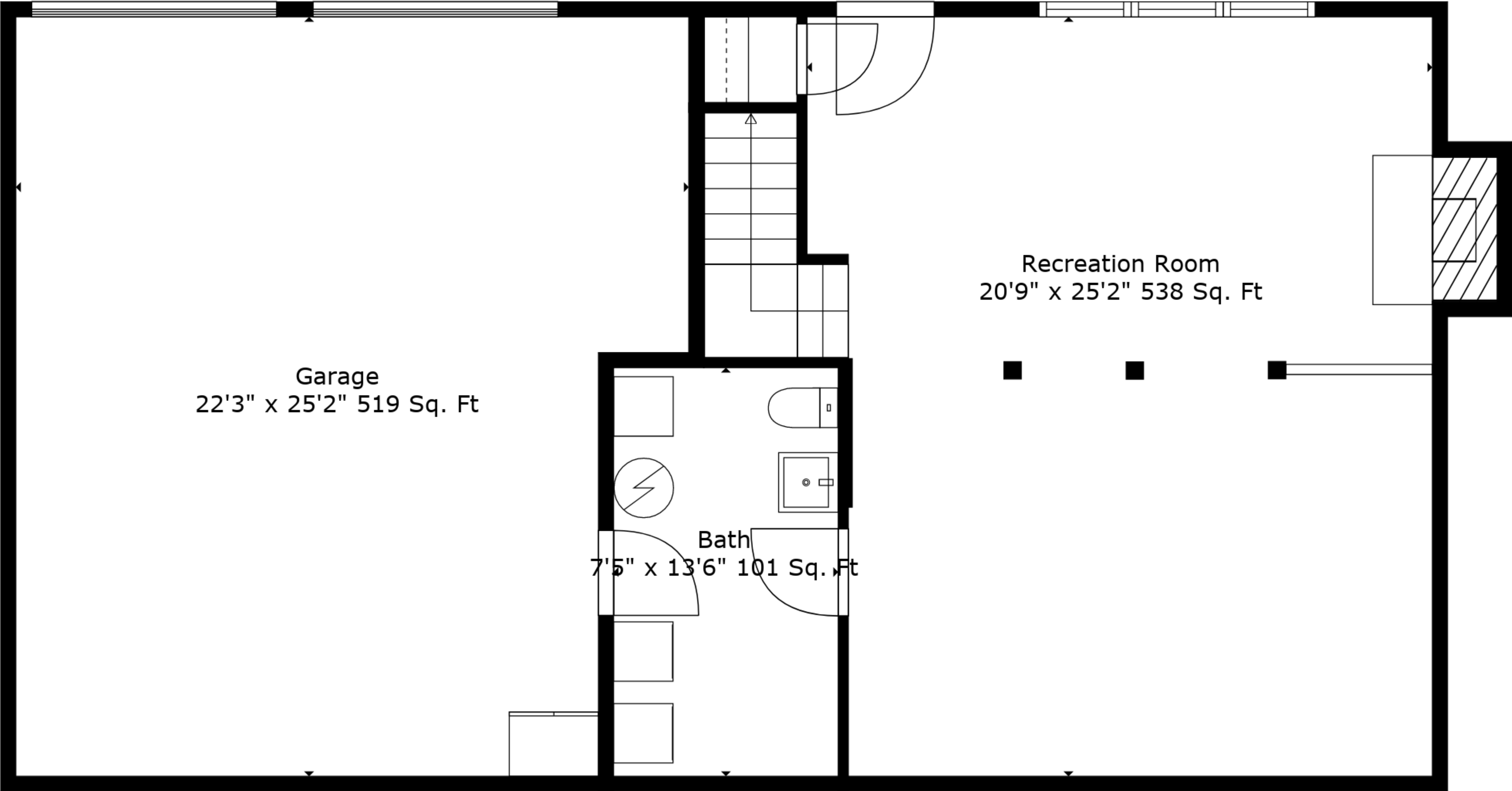
Floor 1
