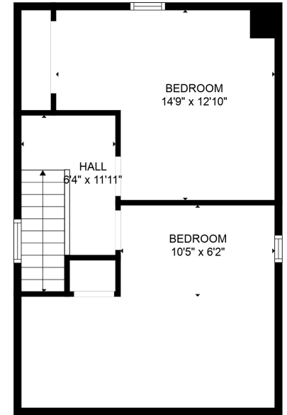
FLOOR 4
