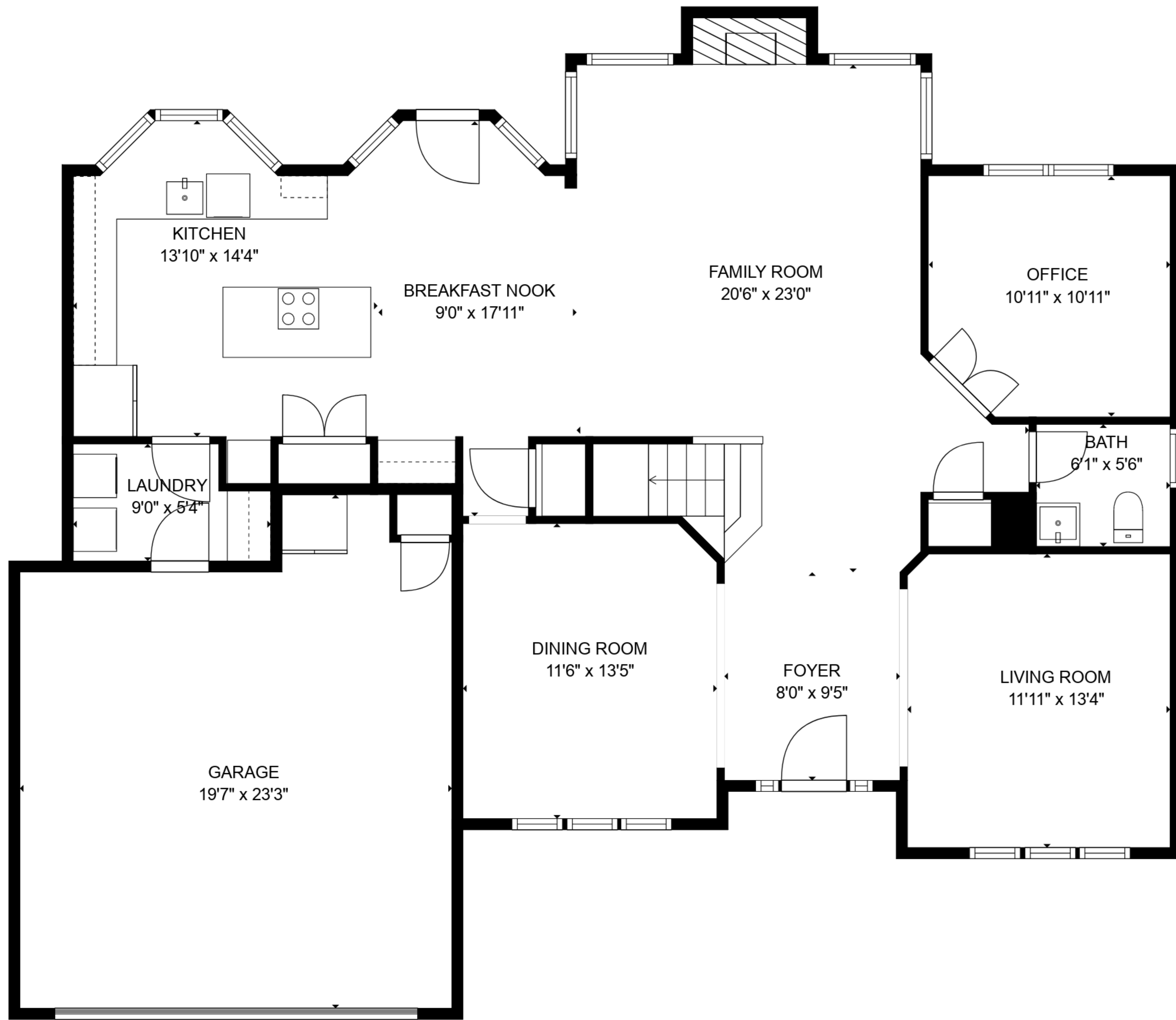
FLOOR 1
