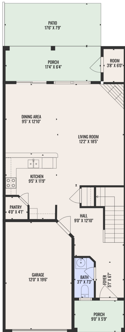
FLOOR 1
