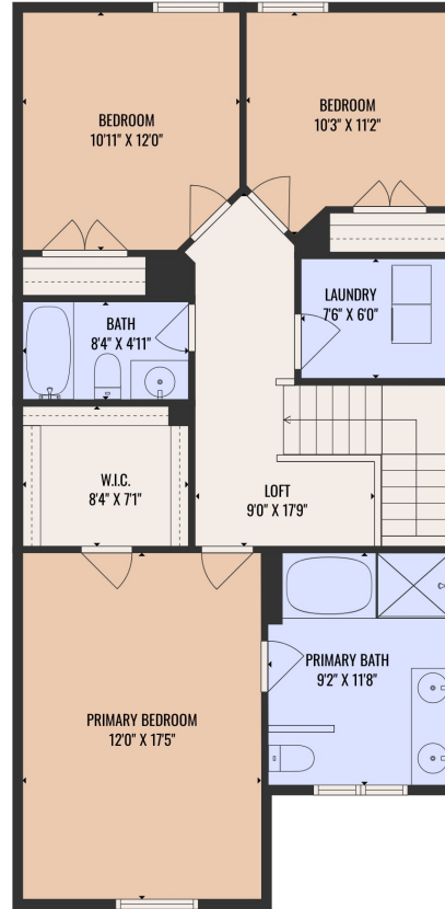
FLOOR 2
