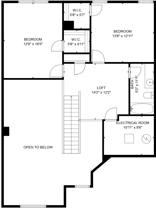
FLOOR 2
