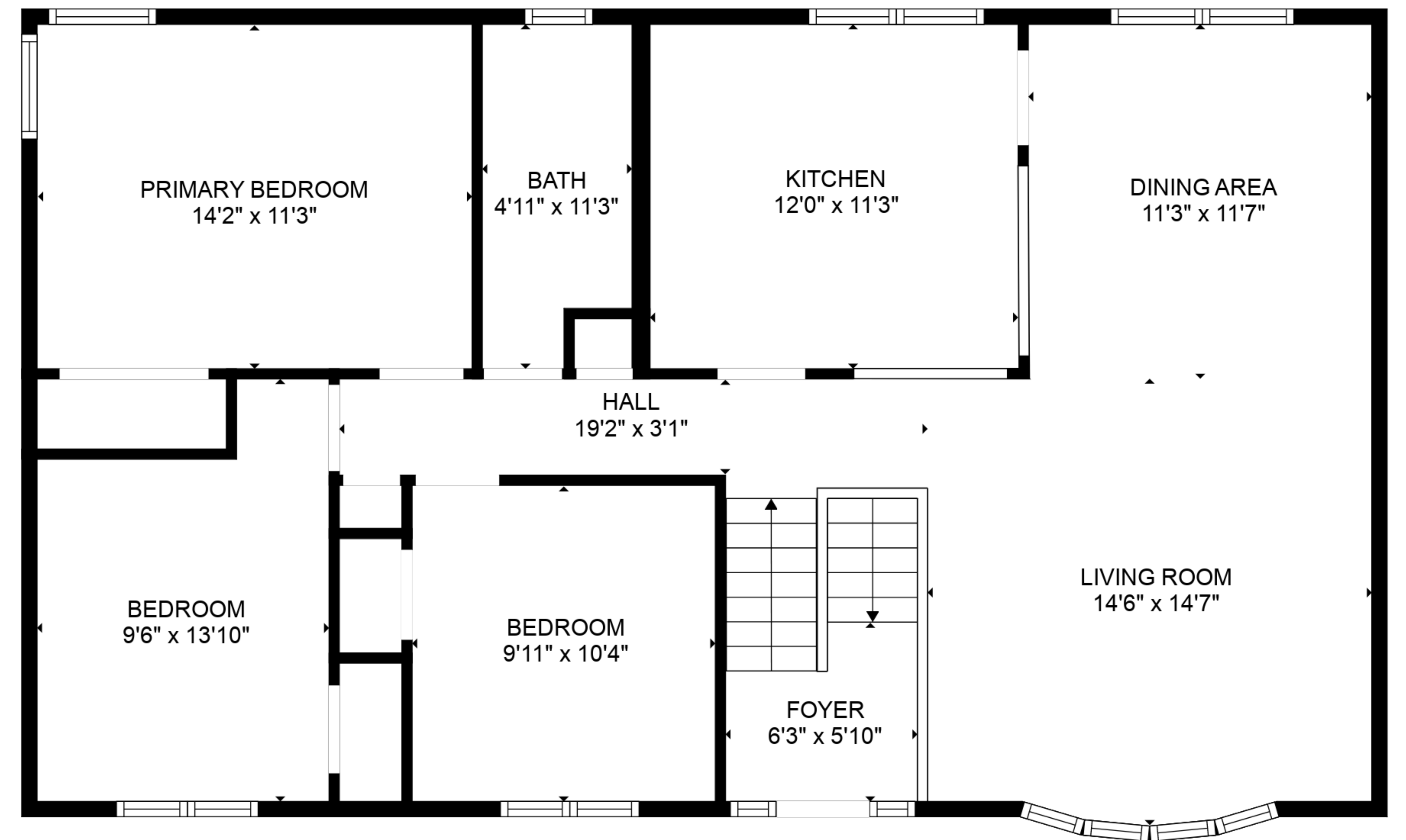
FLOOR 2
