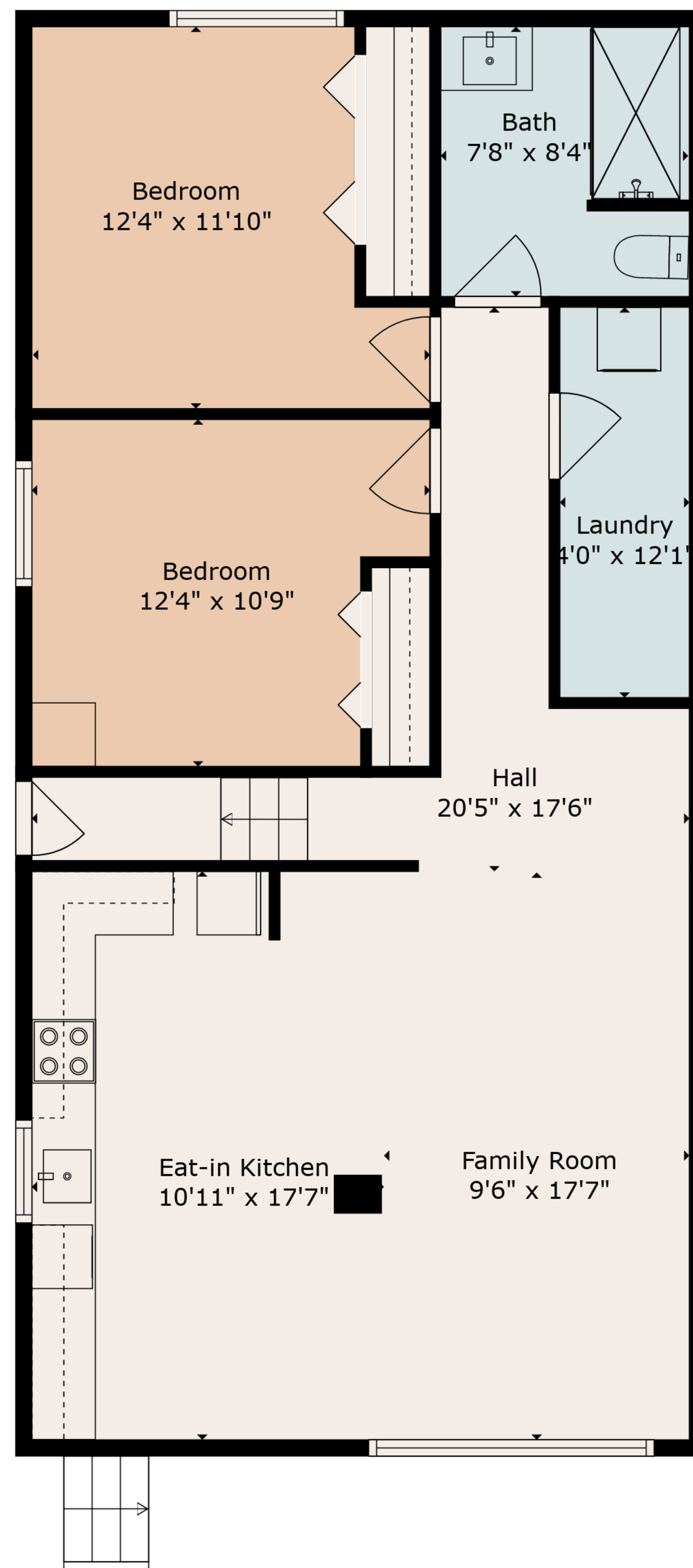
Floor 1
