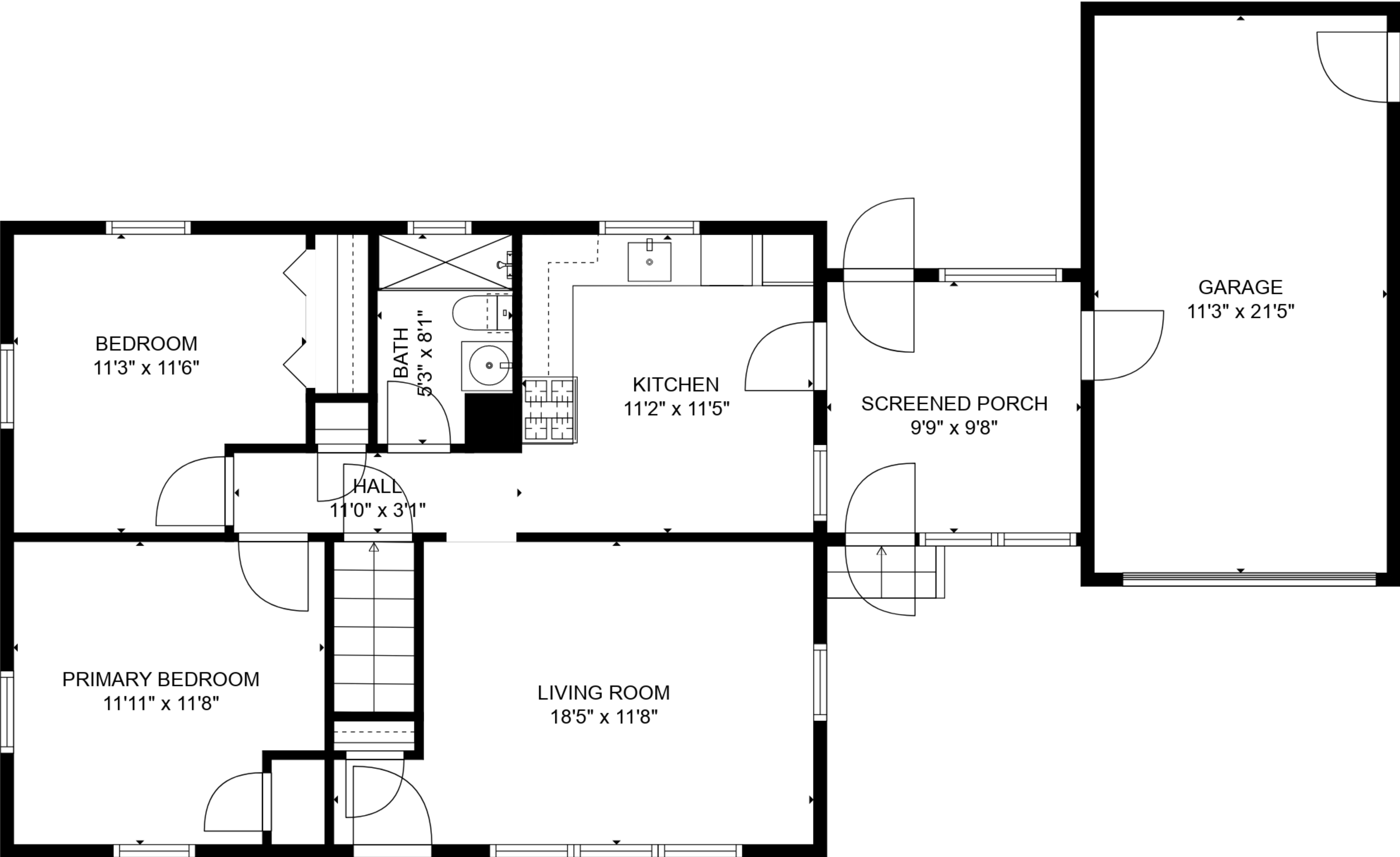
FLOOR 2
