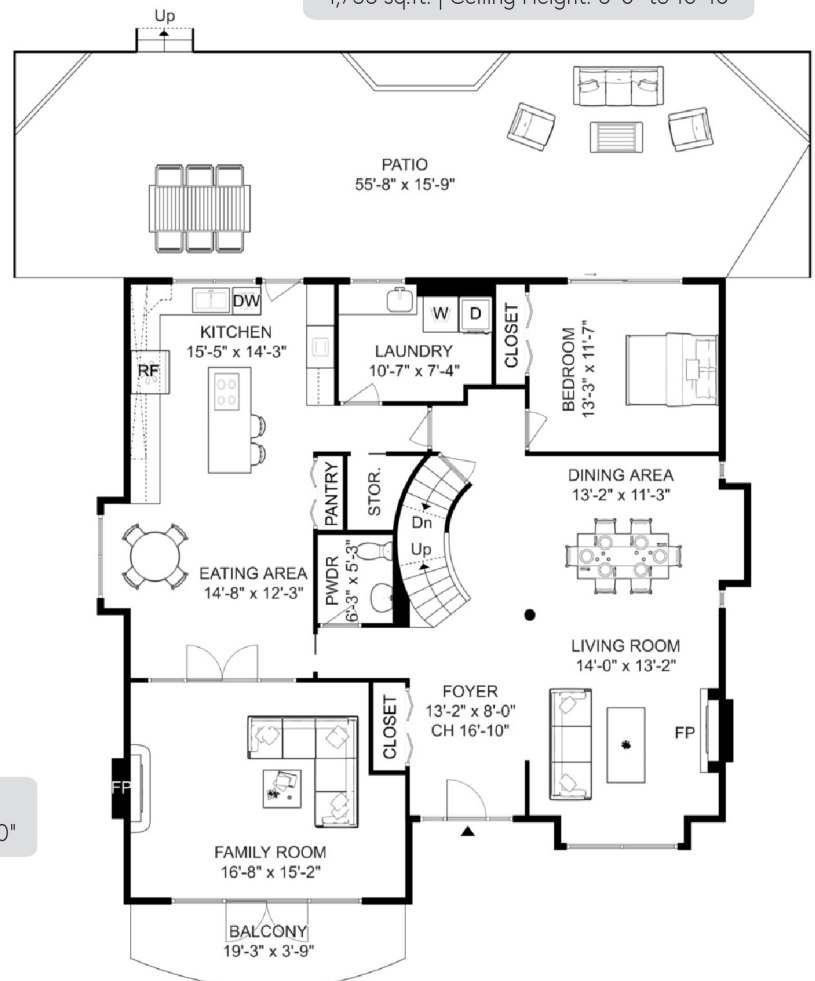
MAIN FLOOR 1,758 sq.ft. | Ceiling Height: 8'-0" to 16'-10"
