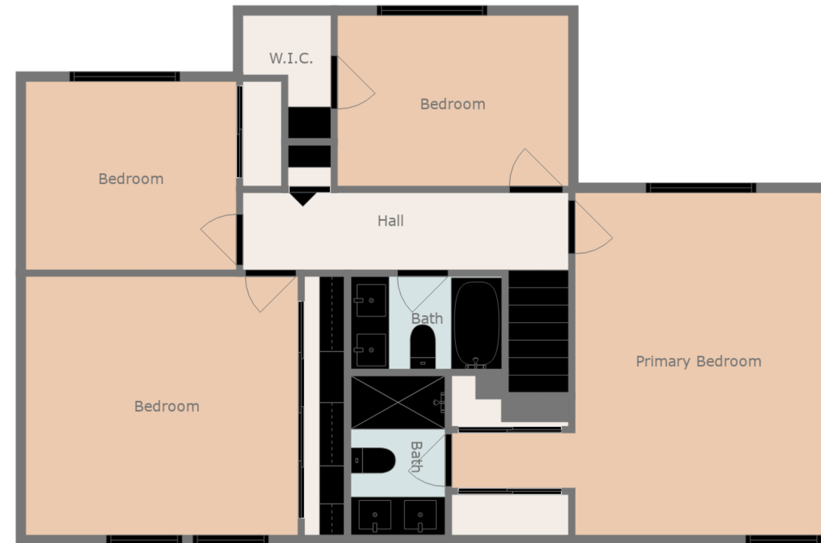
Floor 3
