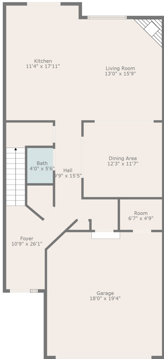
Floor 1
