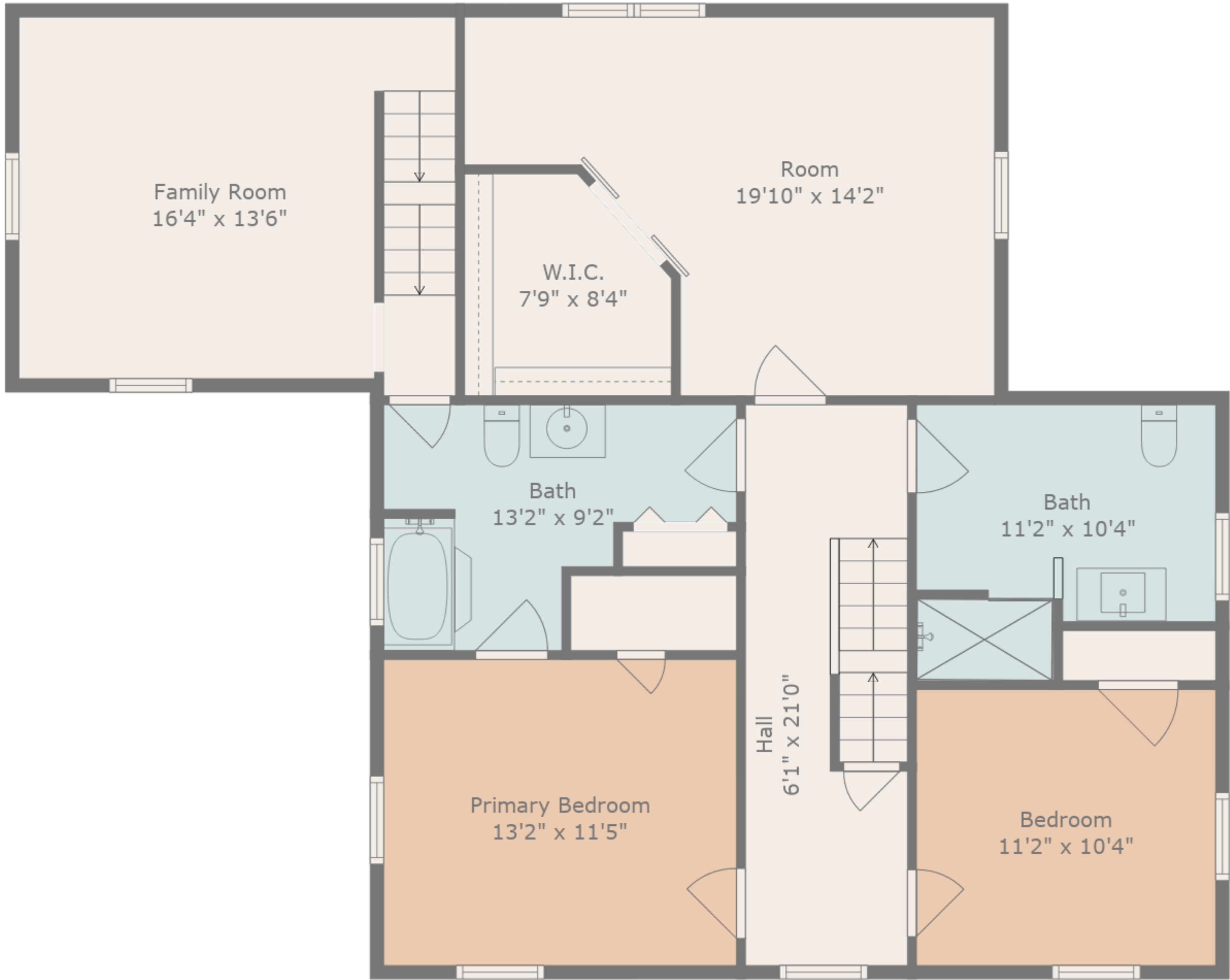
Floor 3
