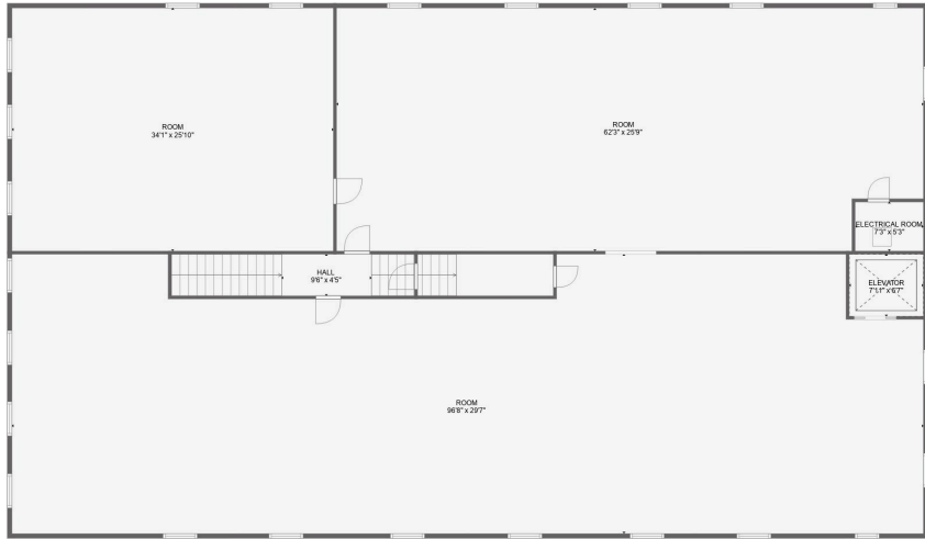
2ND FLOOR
