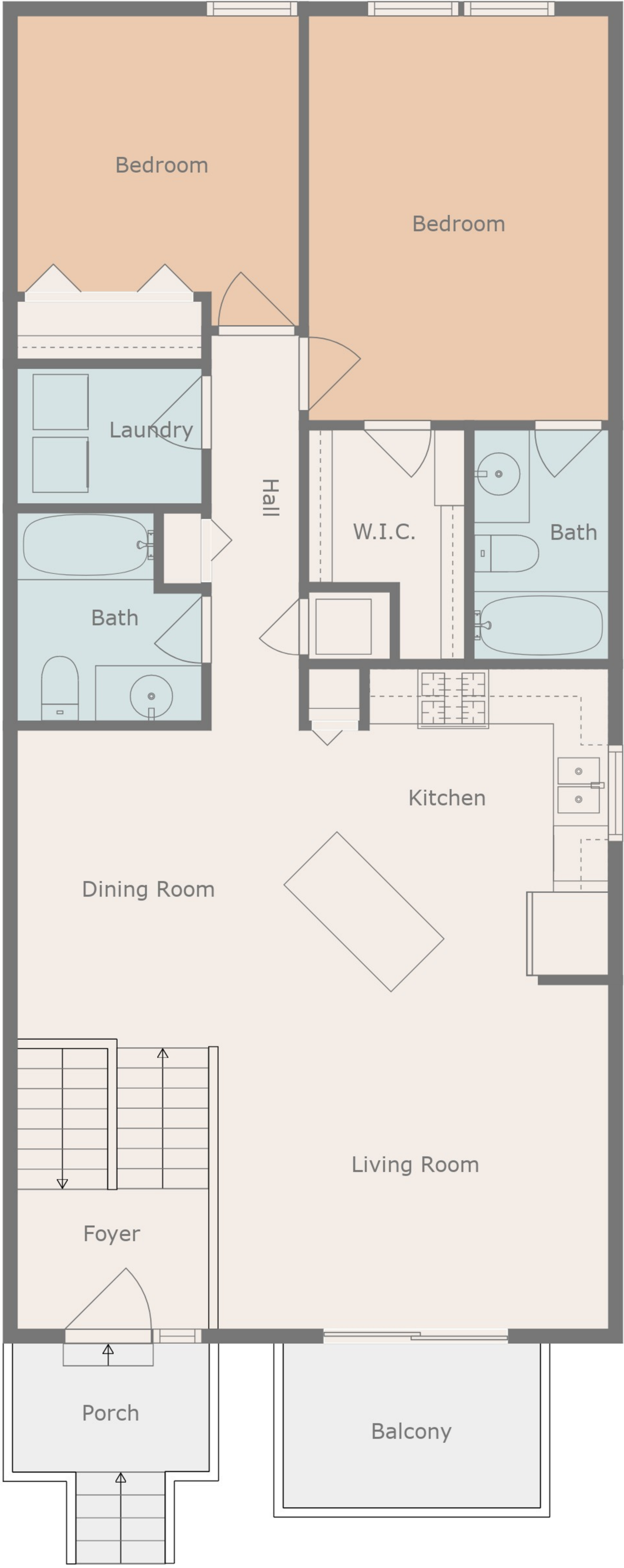
Floor 2
