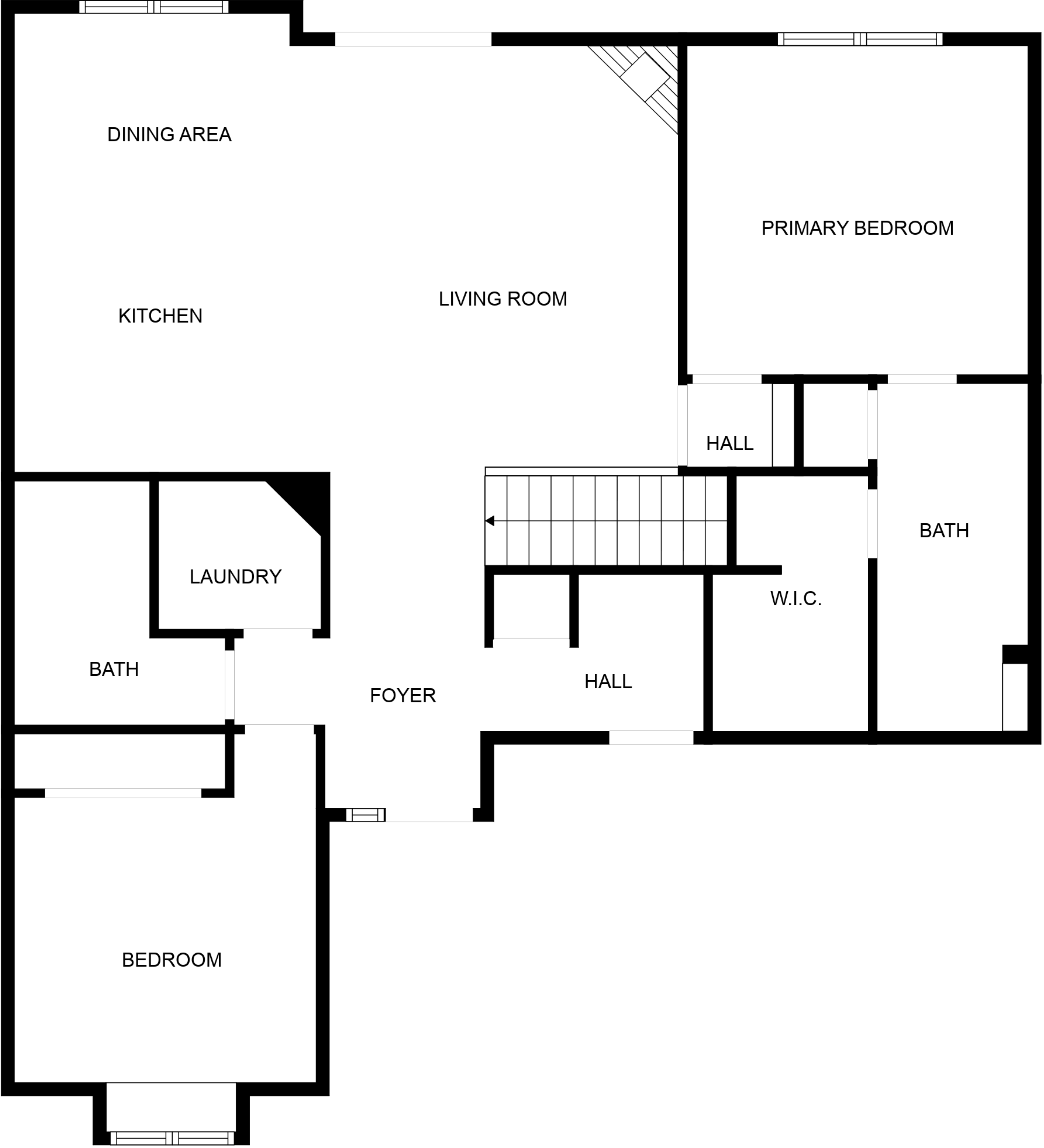
FLOOR 2
