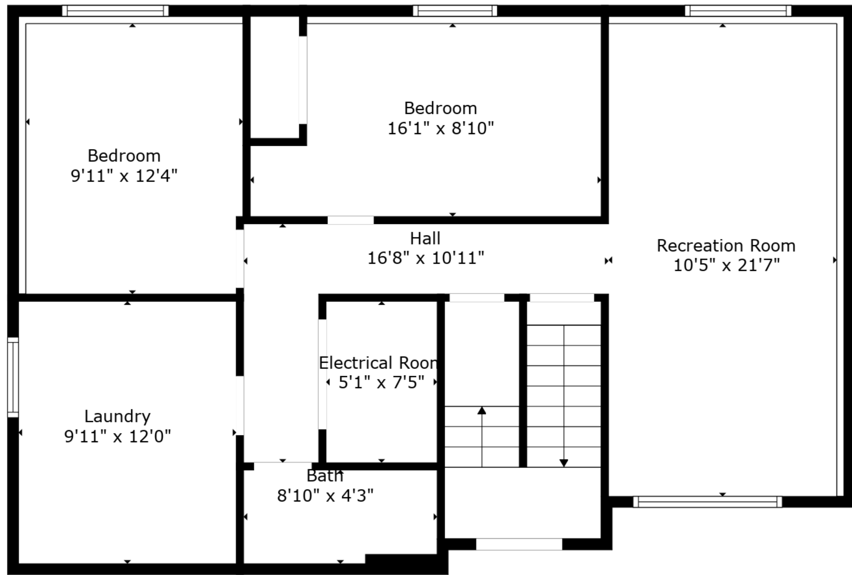
Floor 1
