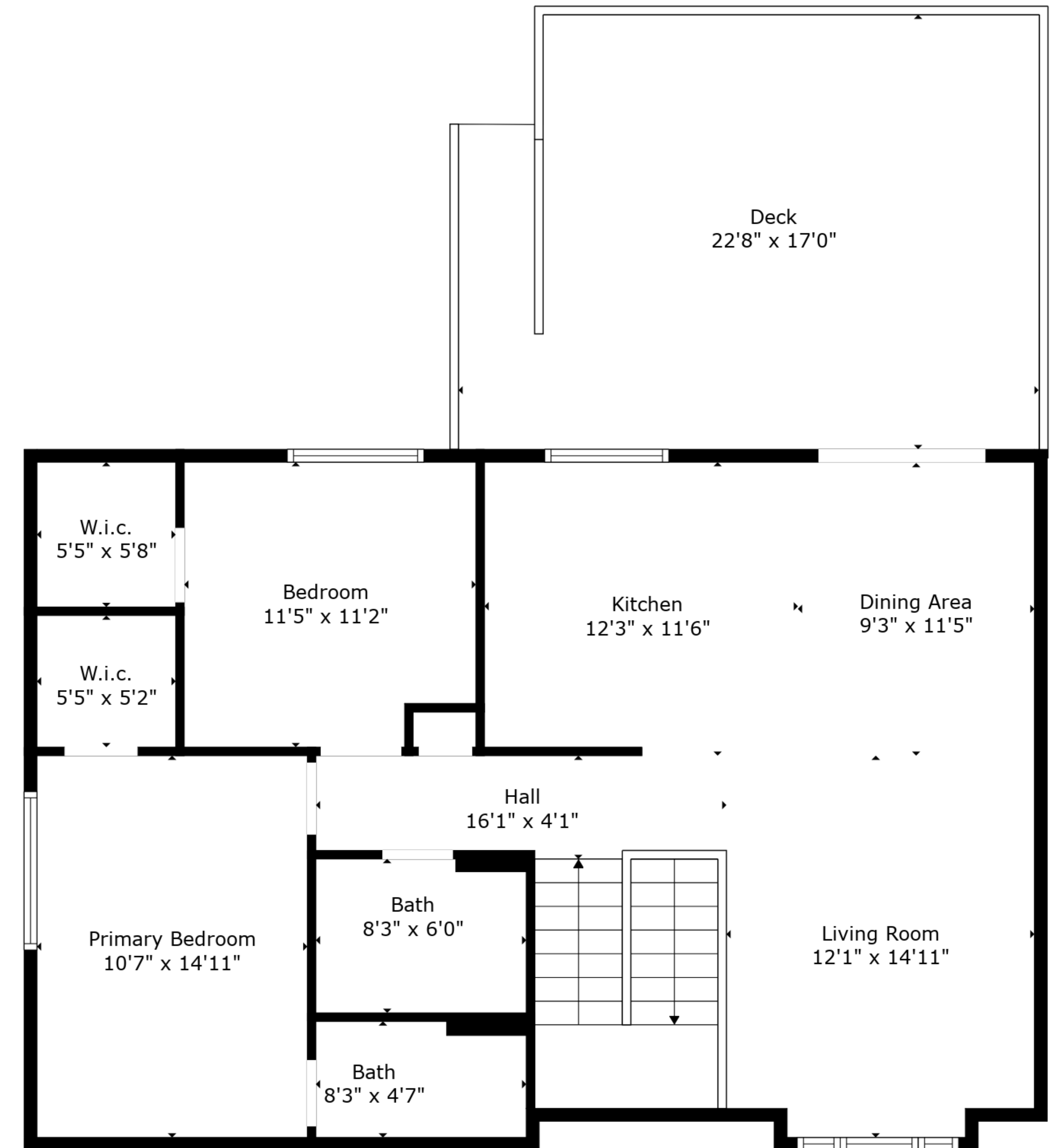
Floor 3
