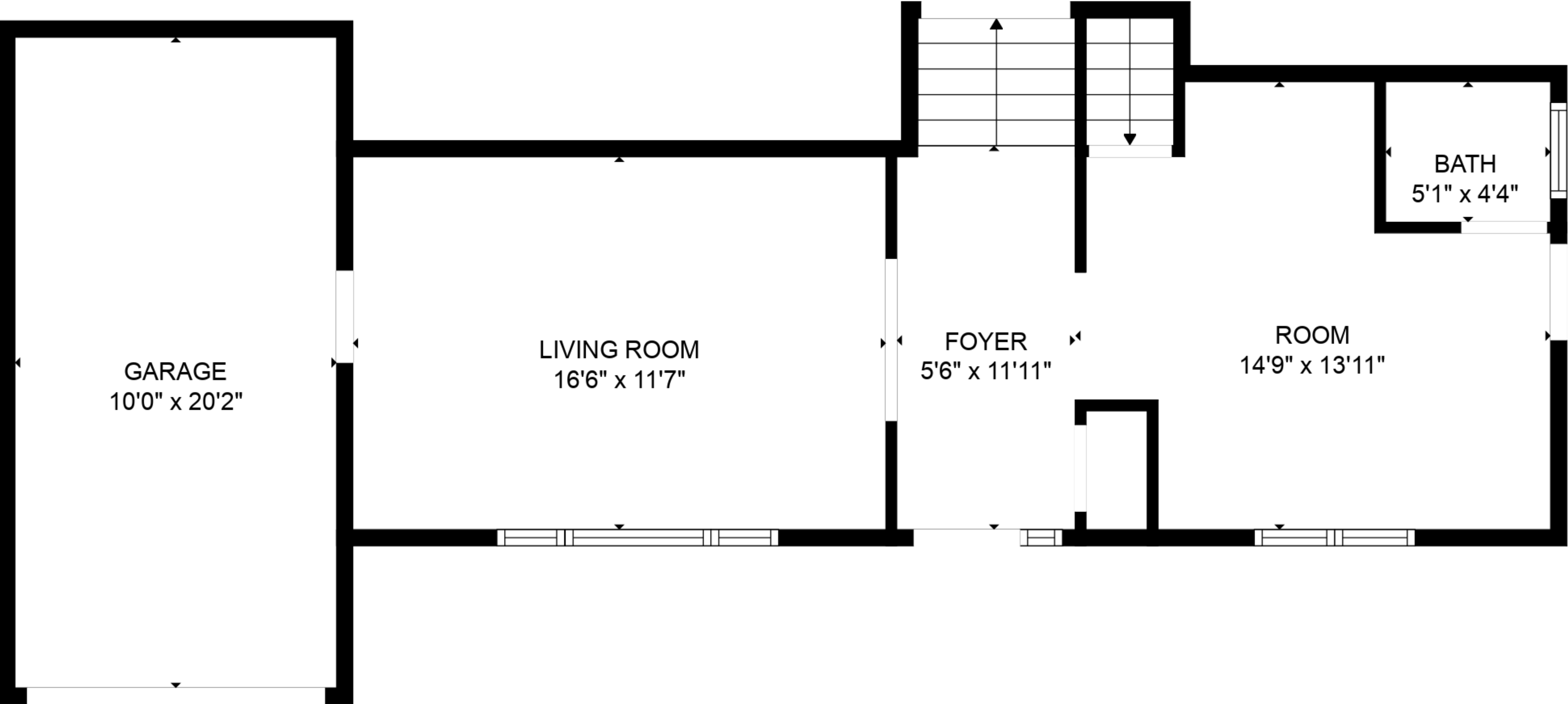
FLOOR 2
