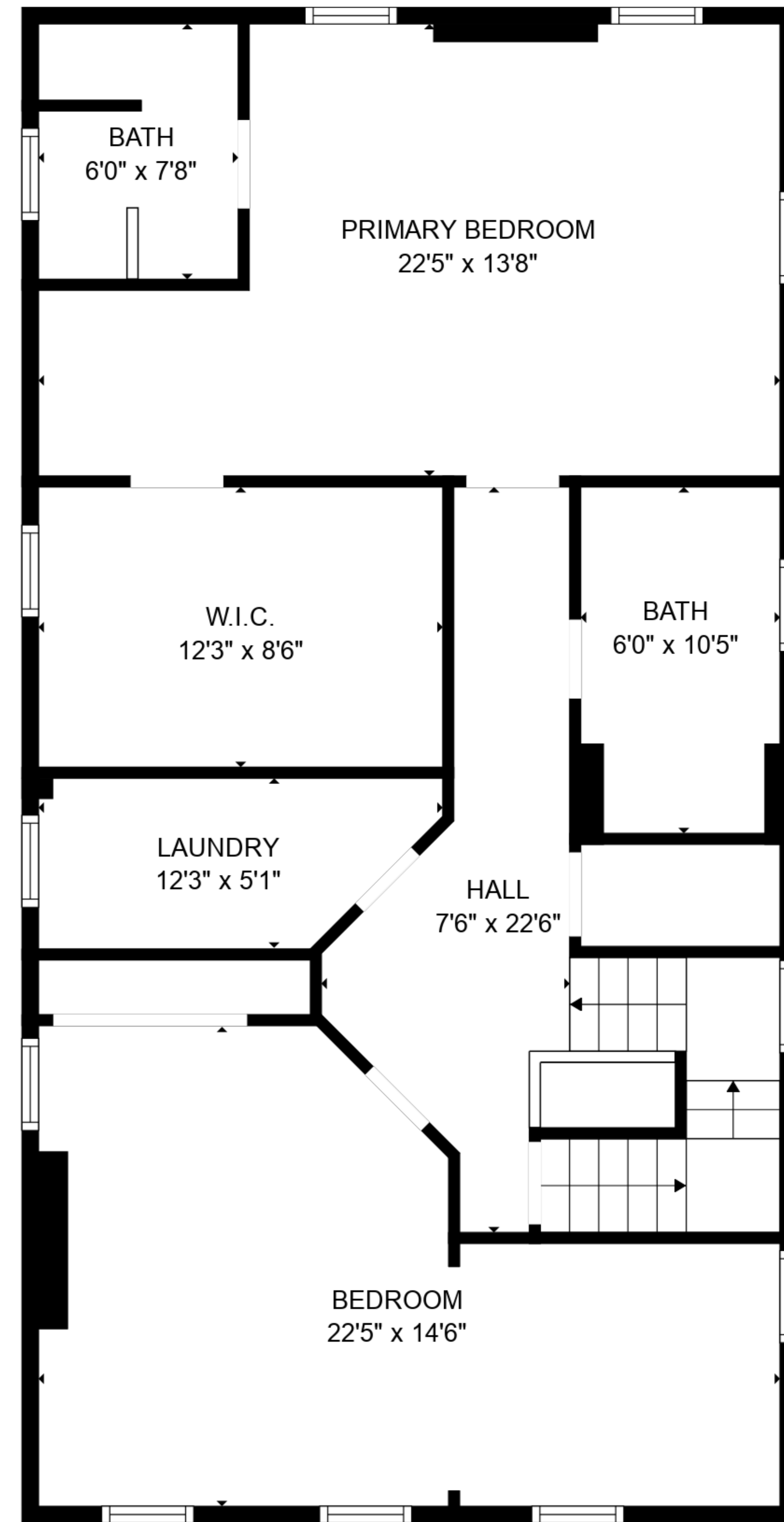
FLOOR 3
