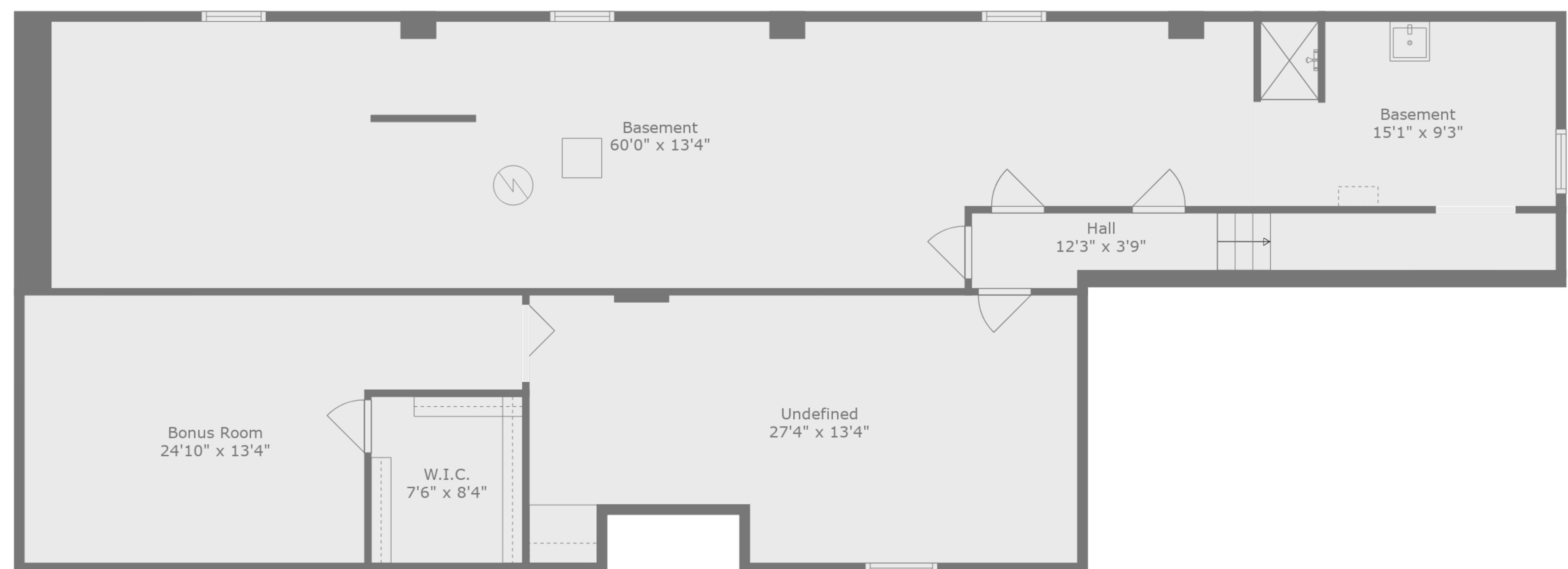
Floor 1
