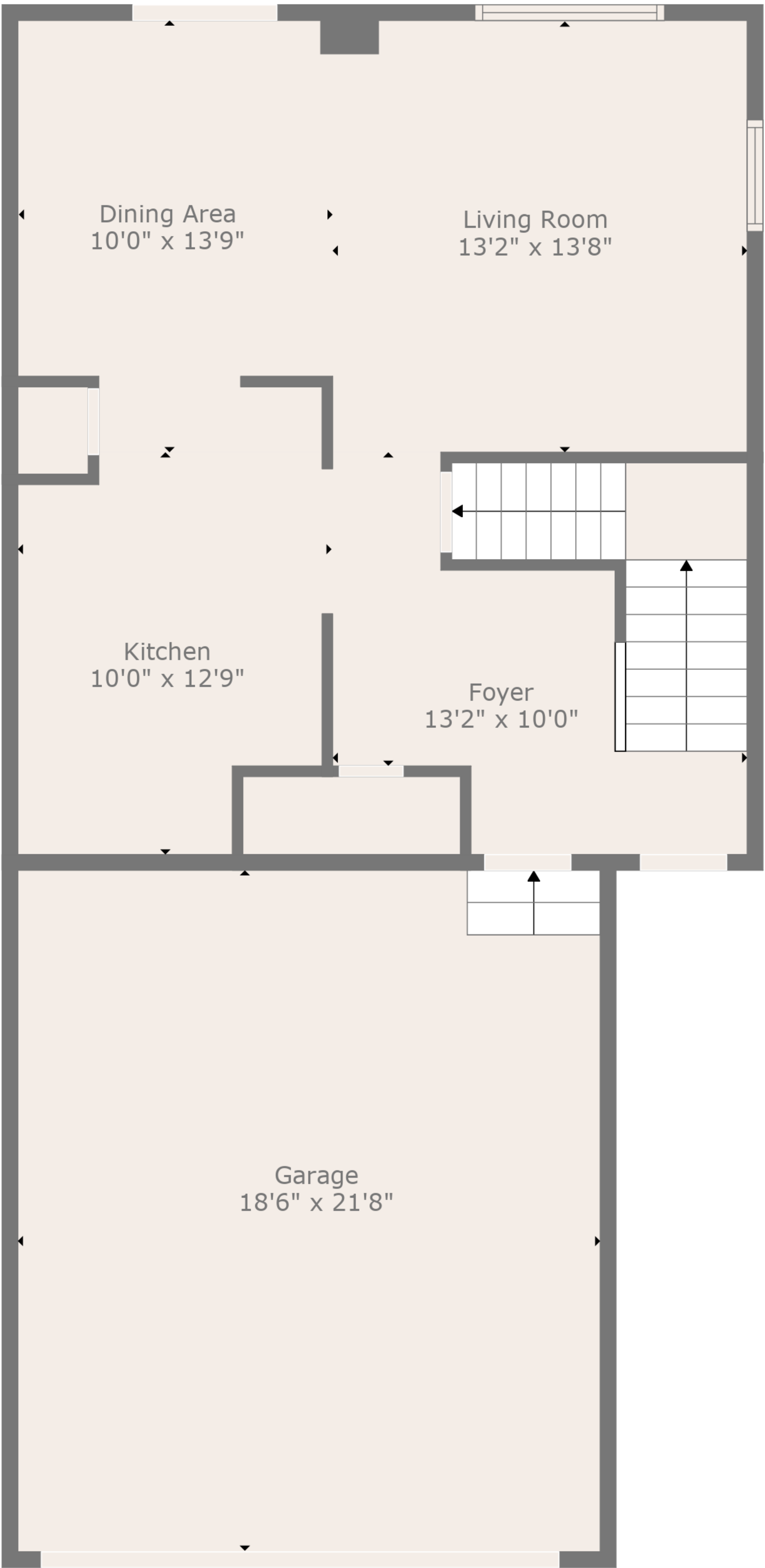
Floor 2
