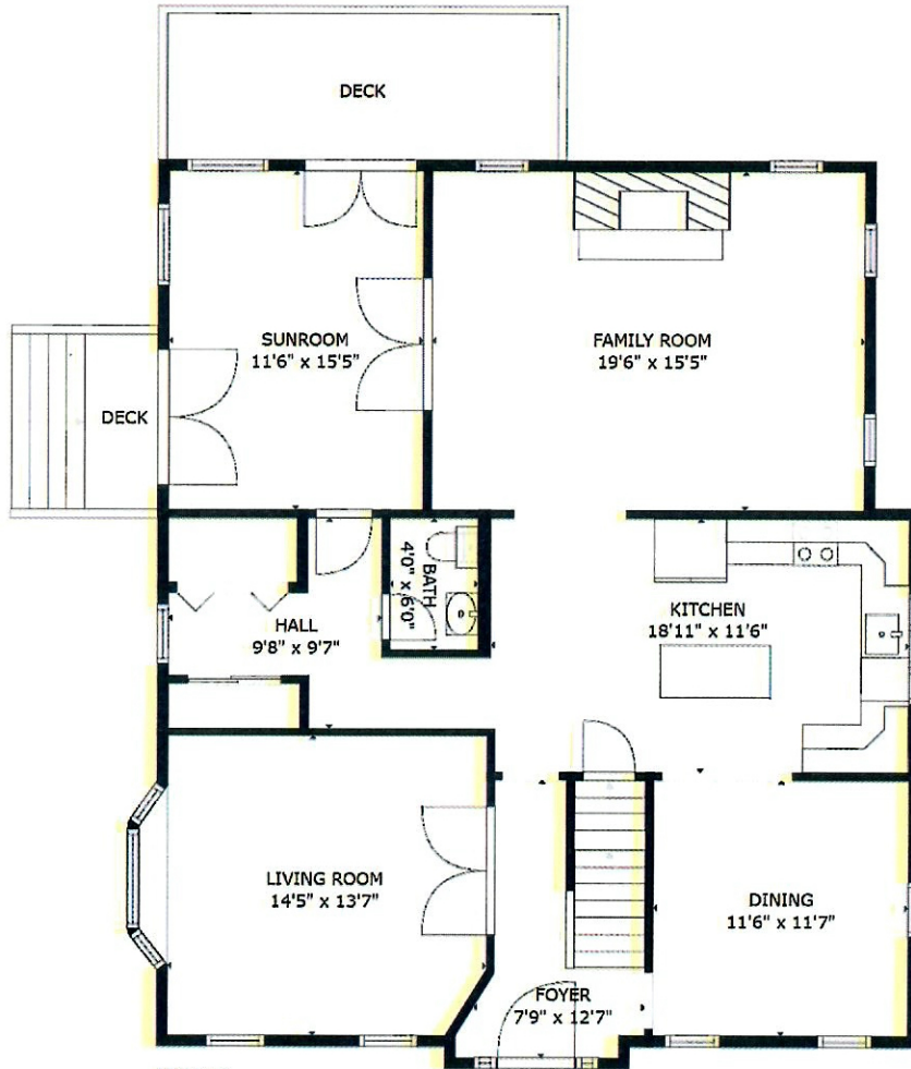
FLOOR 2
