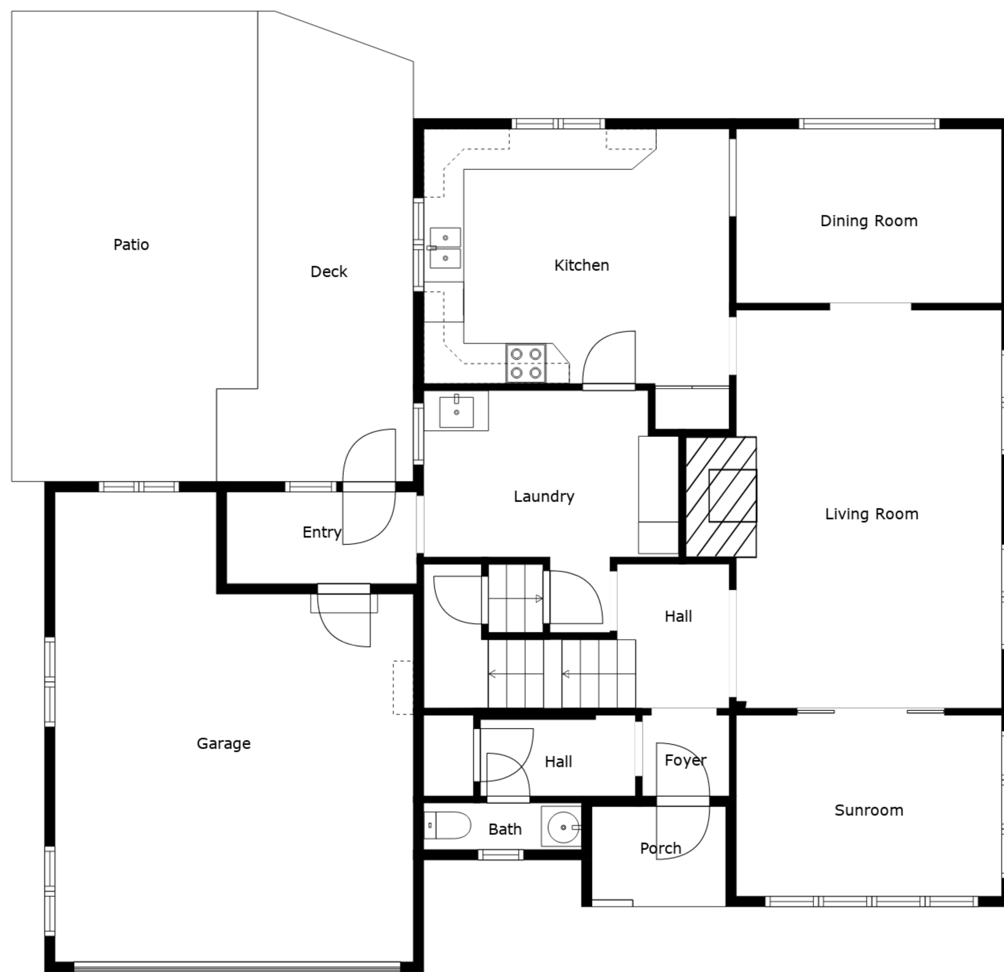
Floor 2
