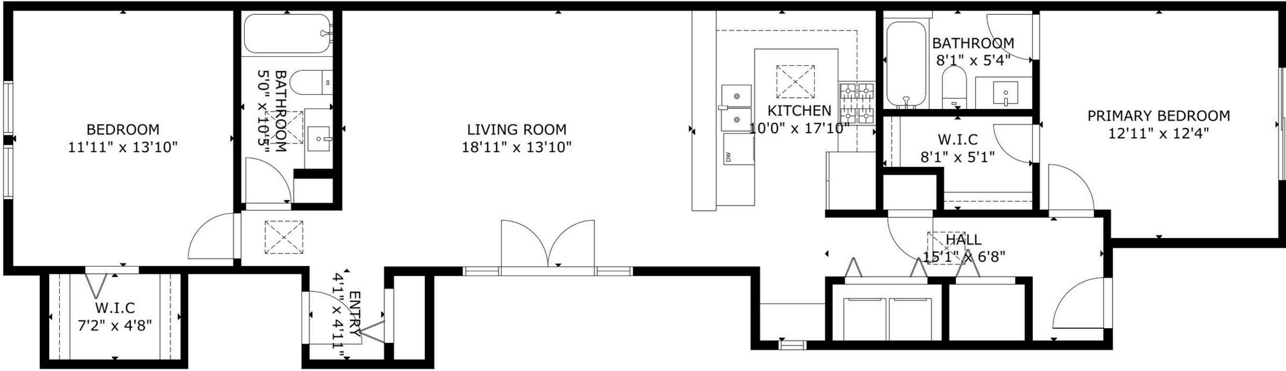
MAIN FLOOR
