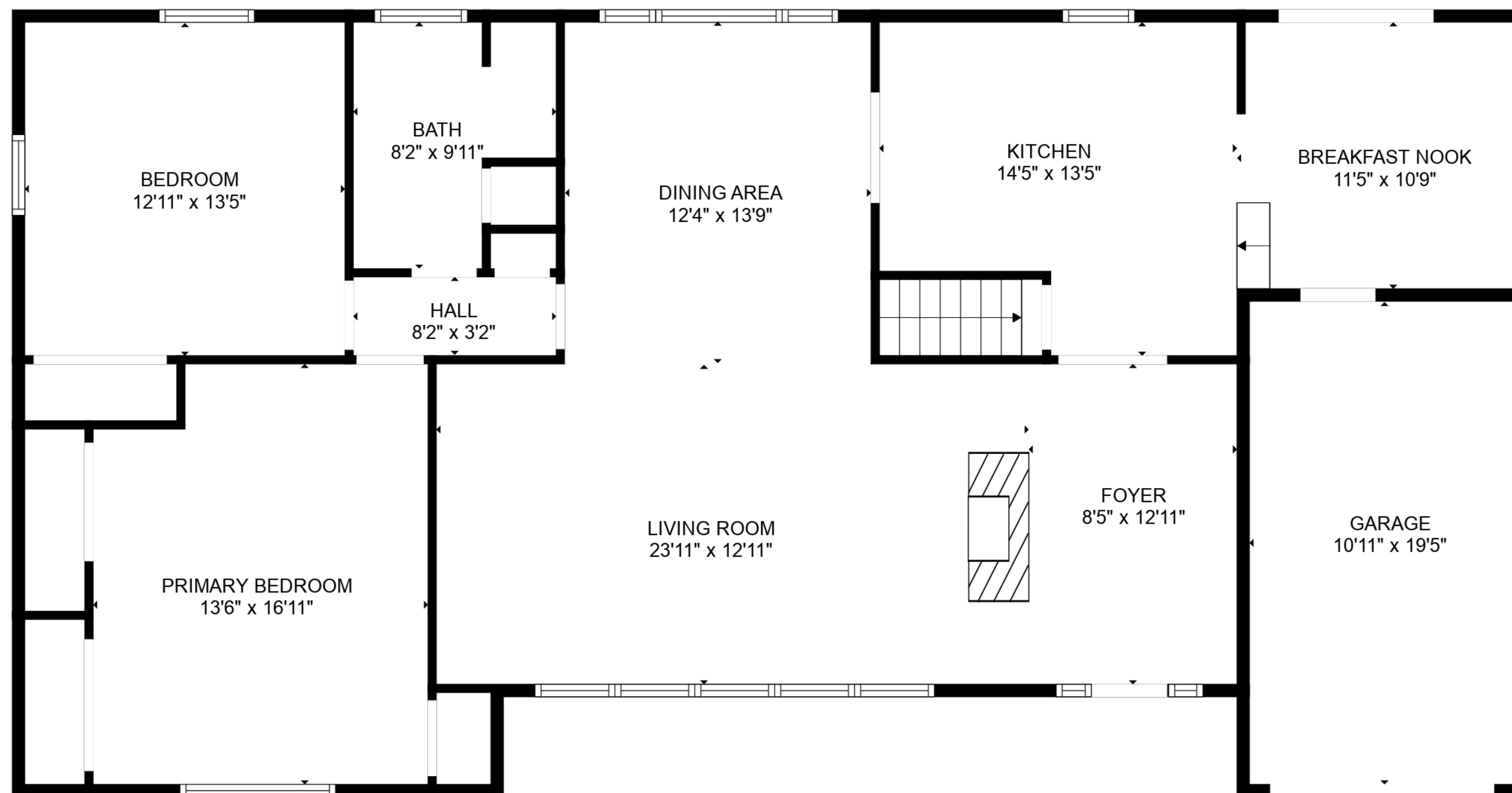
FLOOR 2
