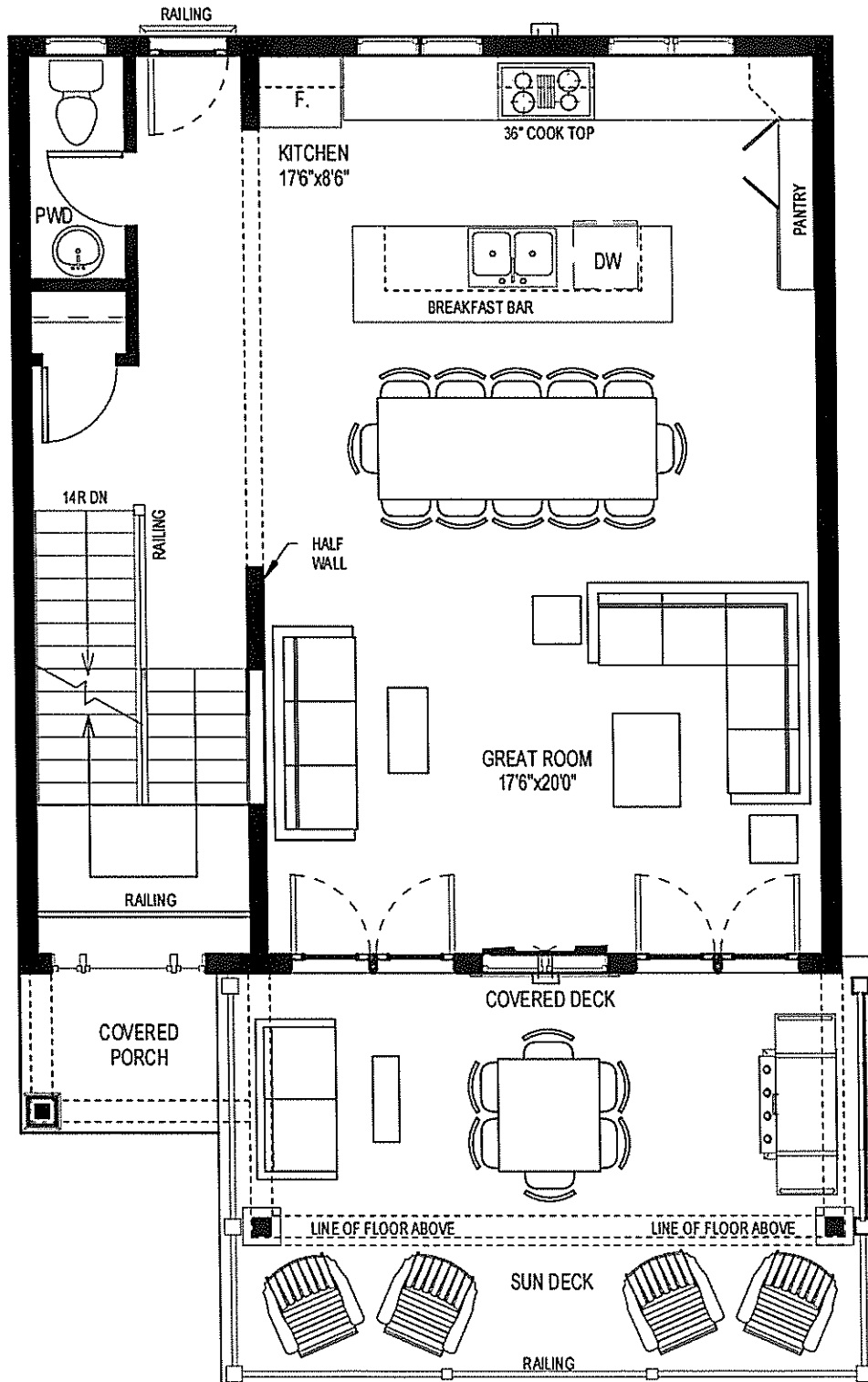
MAIN LEVEL FLOOR PLAN
