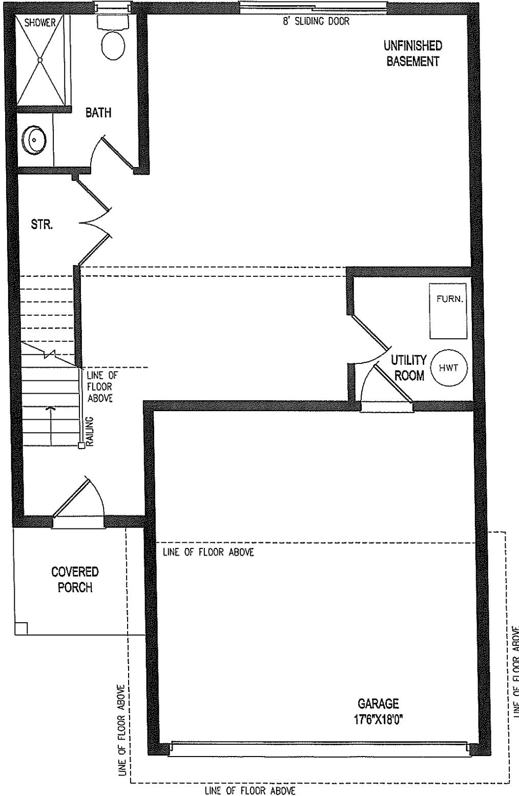
ENTRY LEVEL FLOOR PLAN
