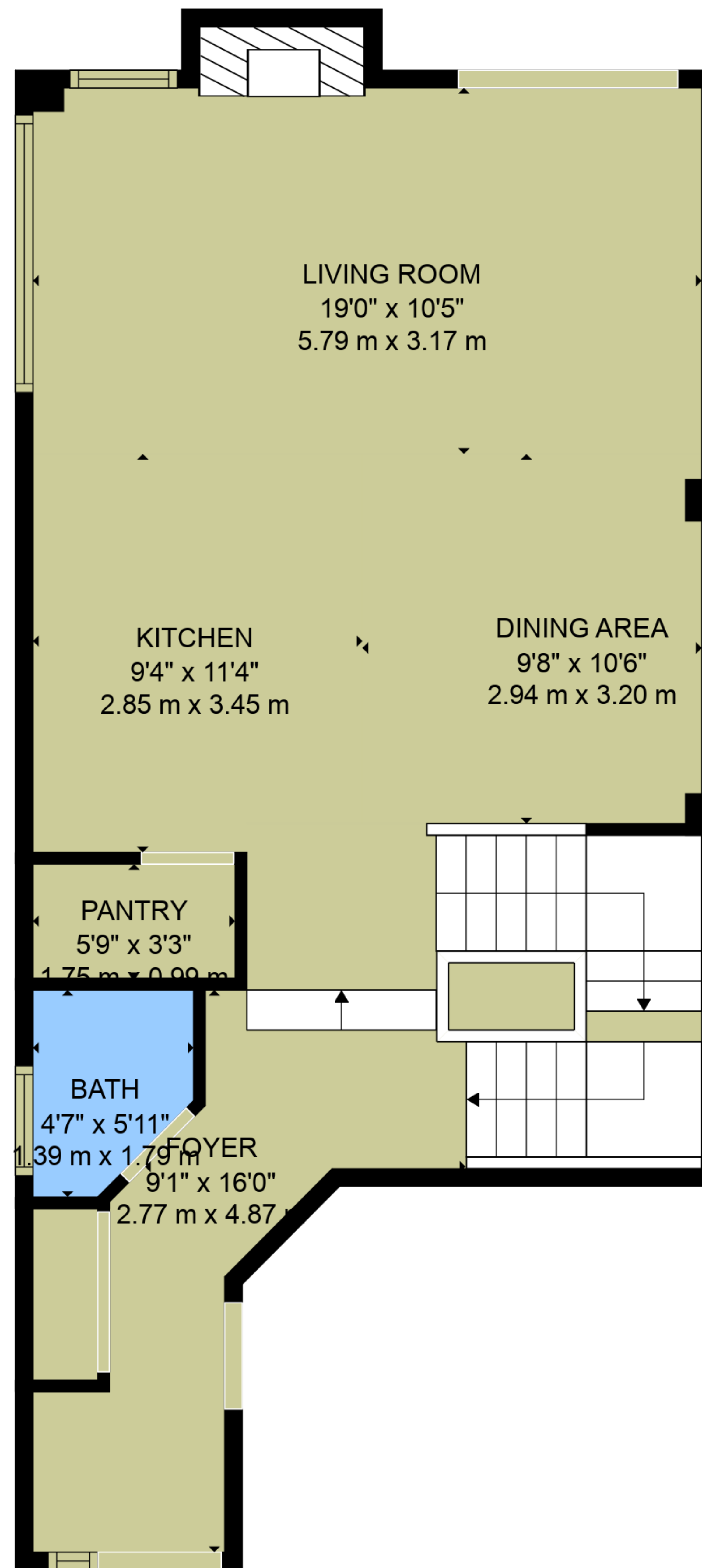
FLOOR 2
