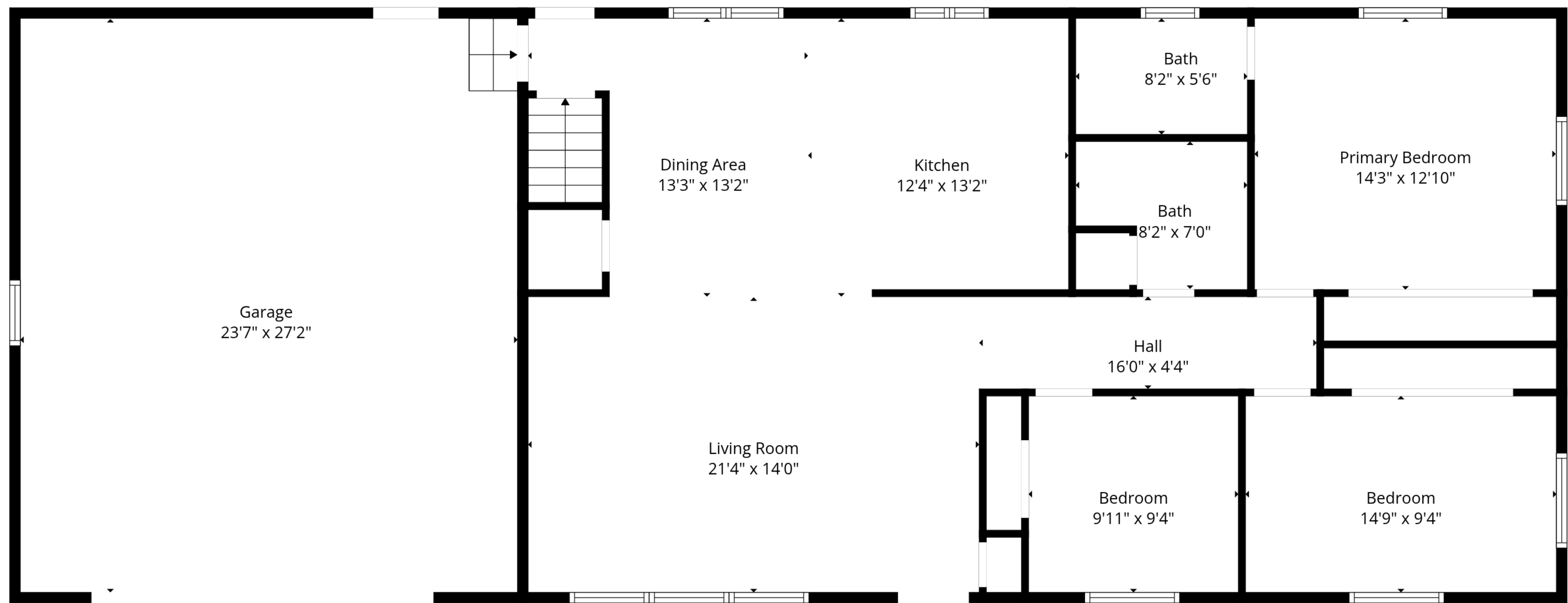
Floor 2
