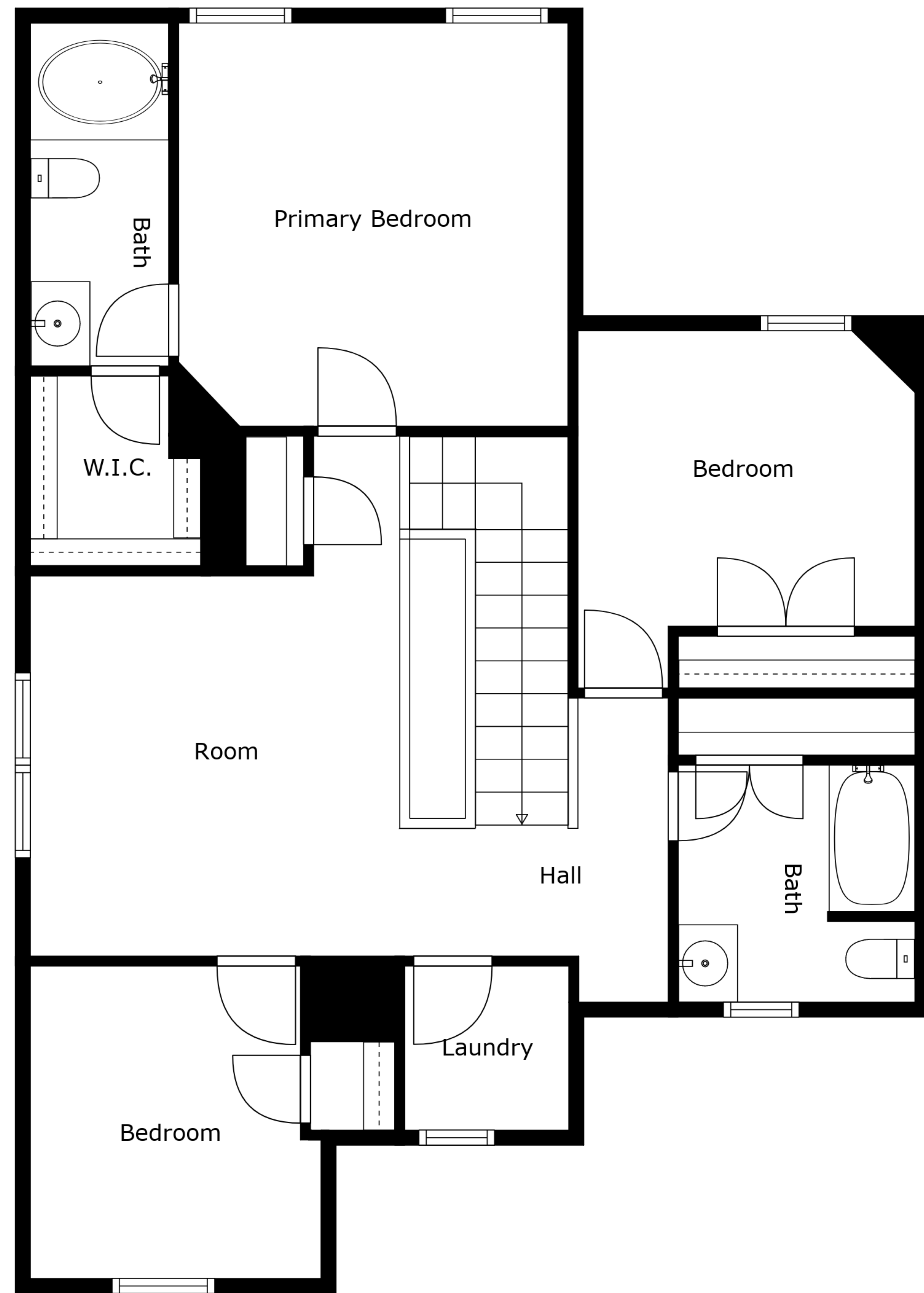
Floor 2
