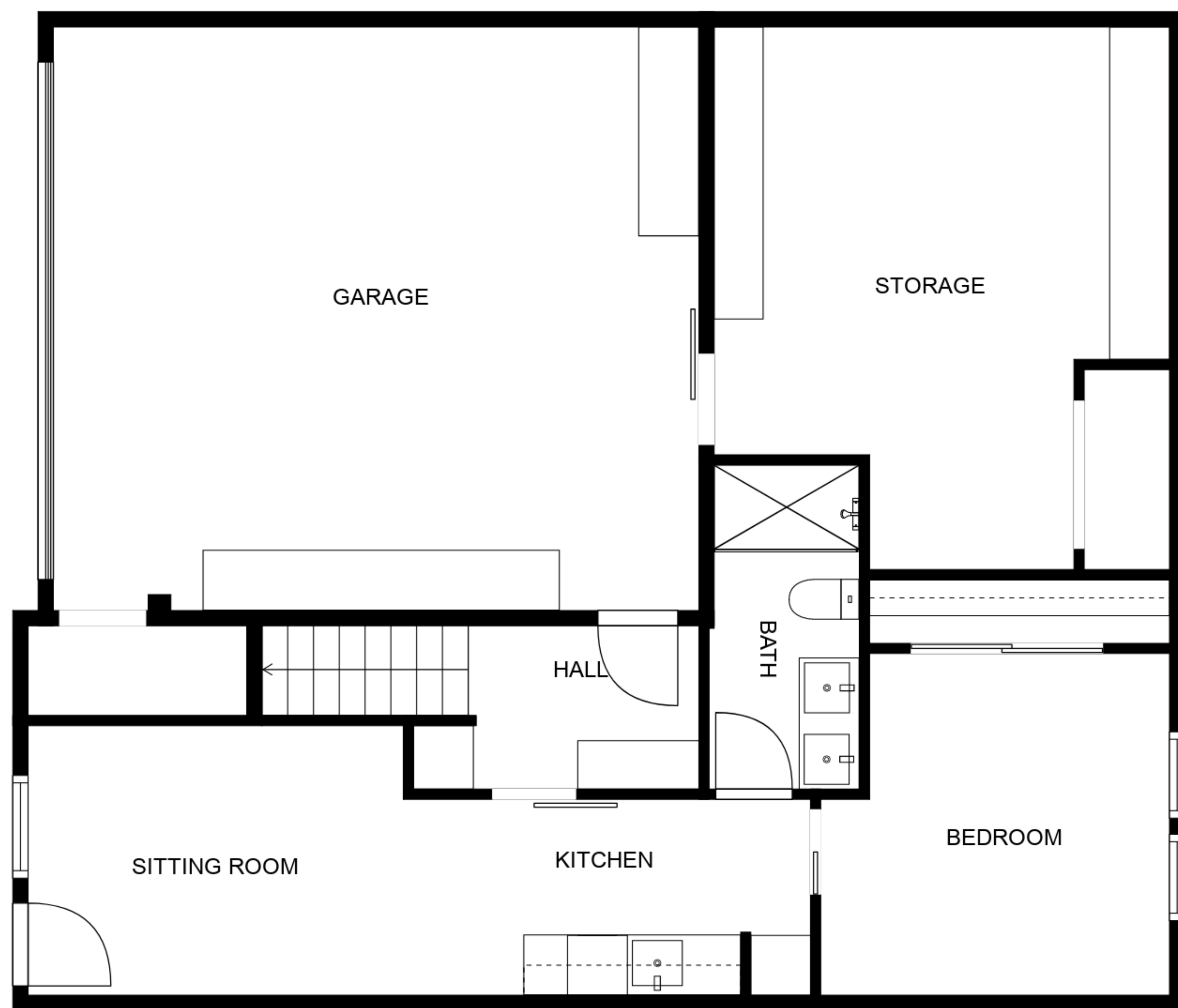
FLOOR 2
