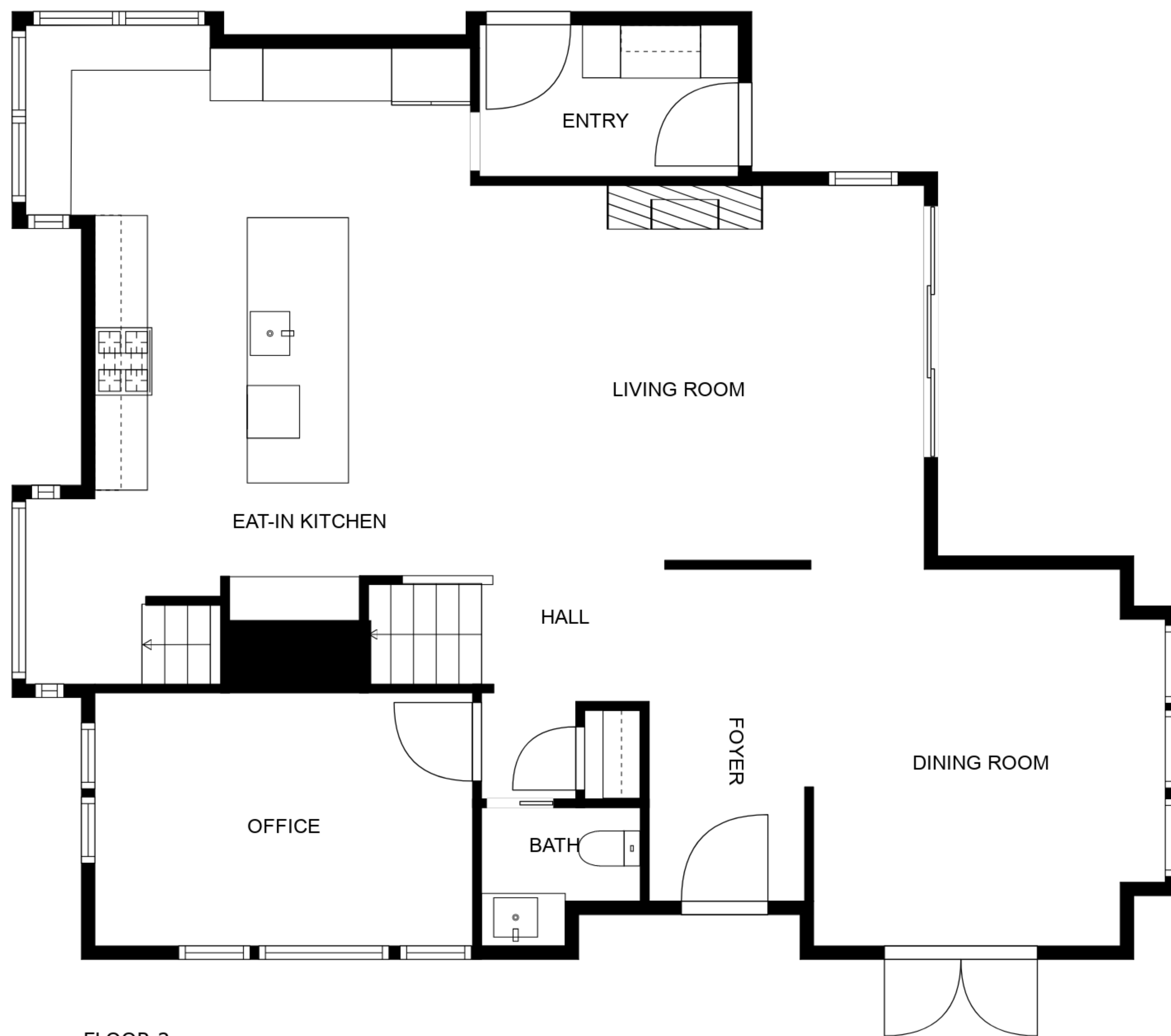
FLOOR 2
