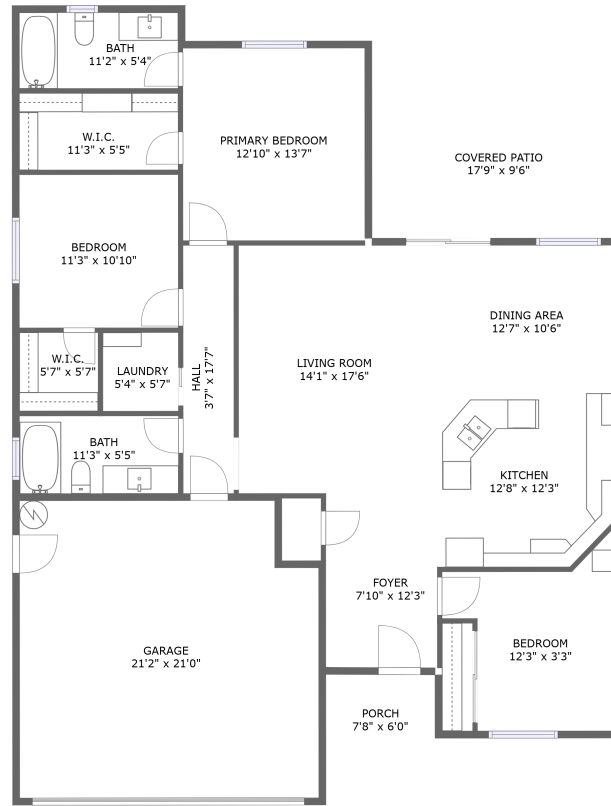
FLOOR 1
