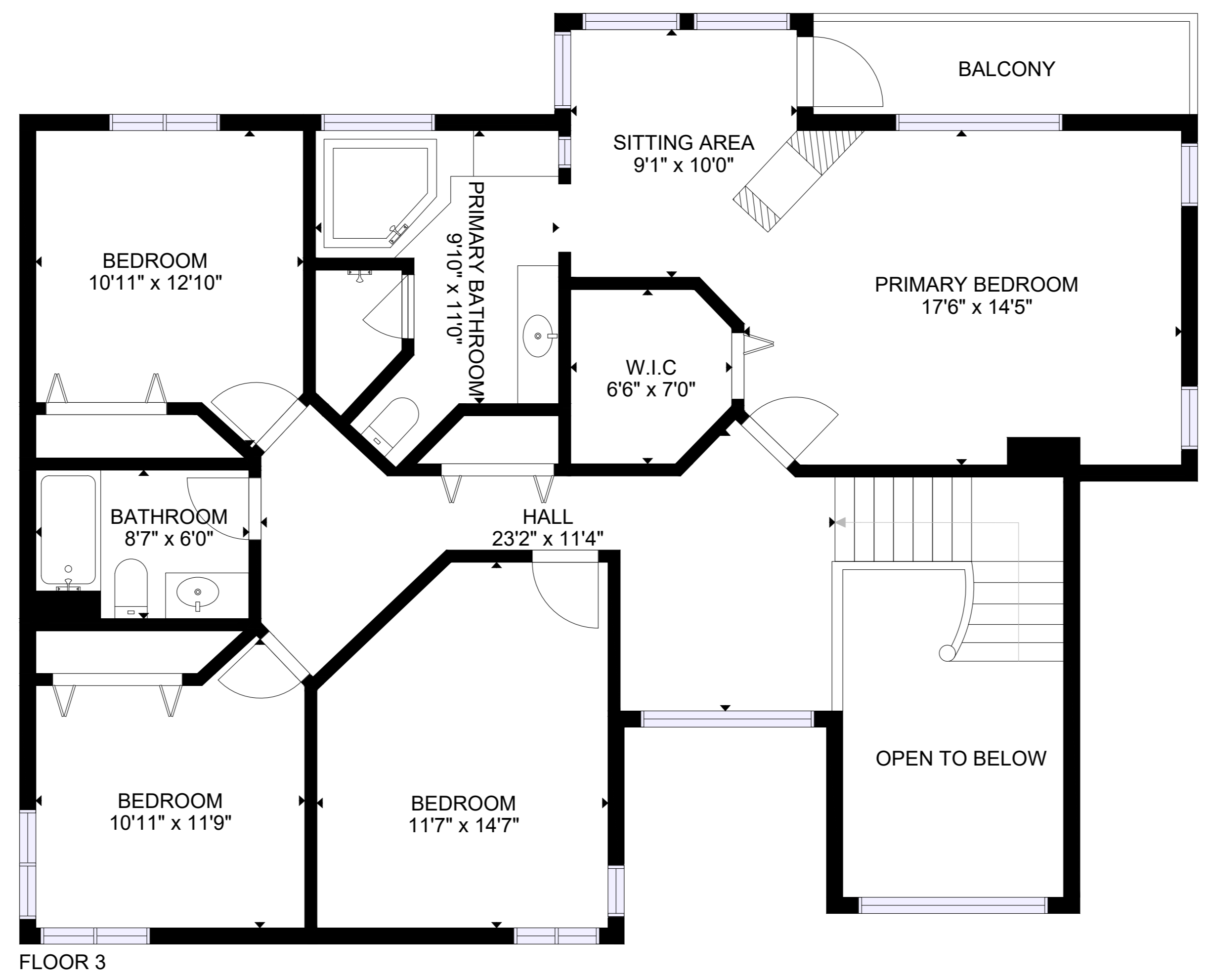
FLOOR 3
