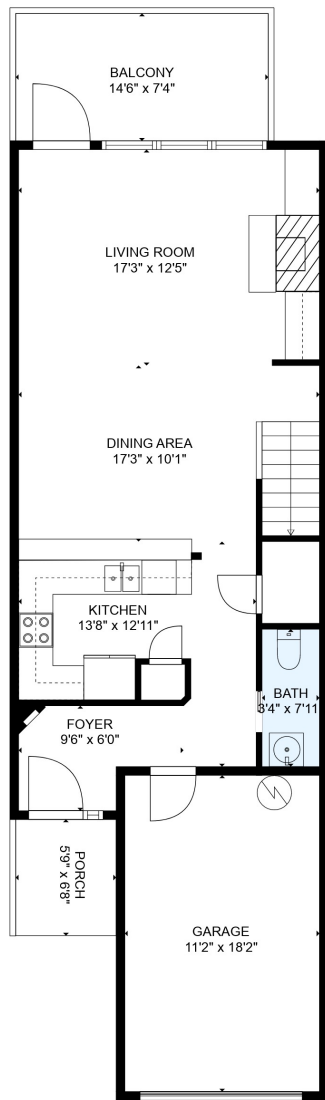
FLOOR 1
