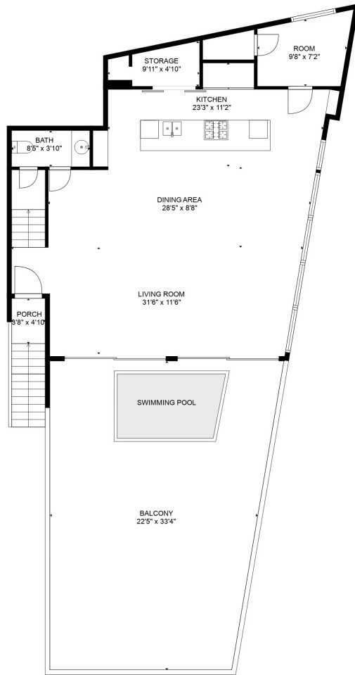
FLOOR 2
