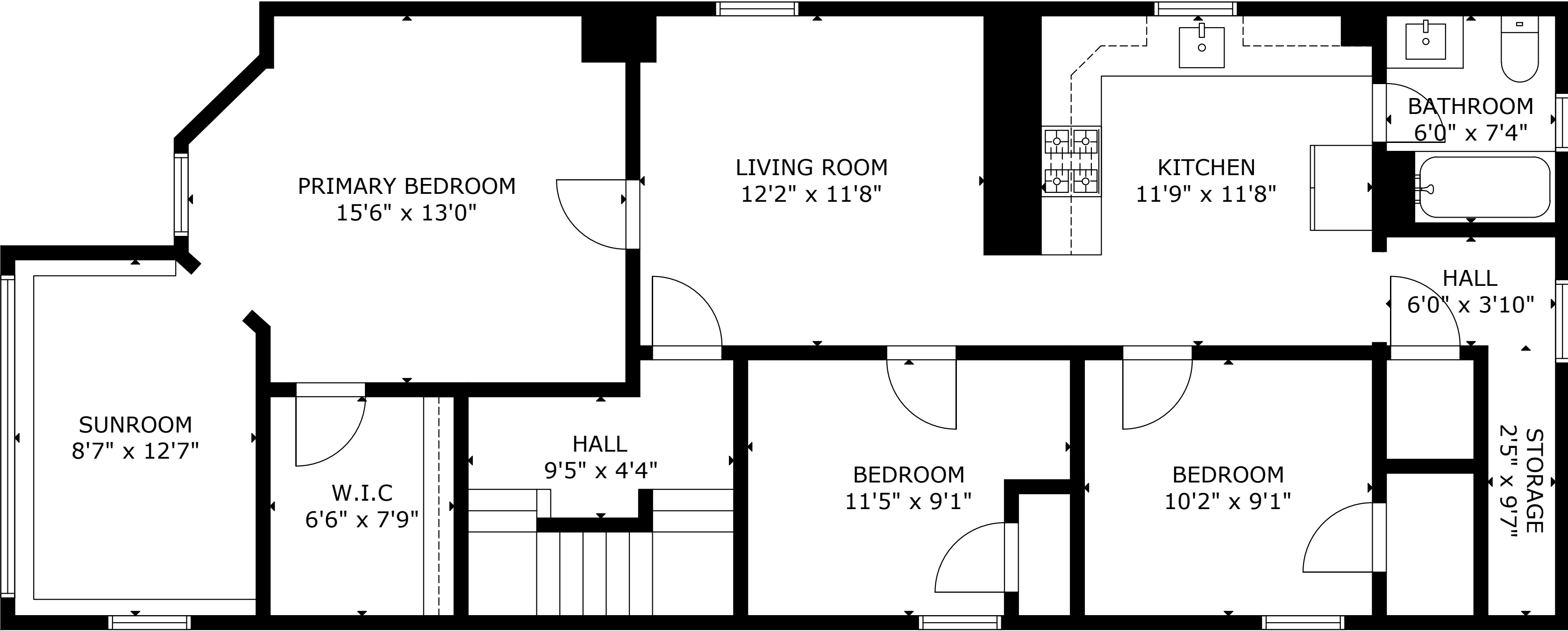
SECOND FLOOR
