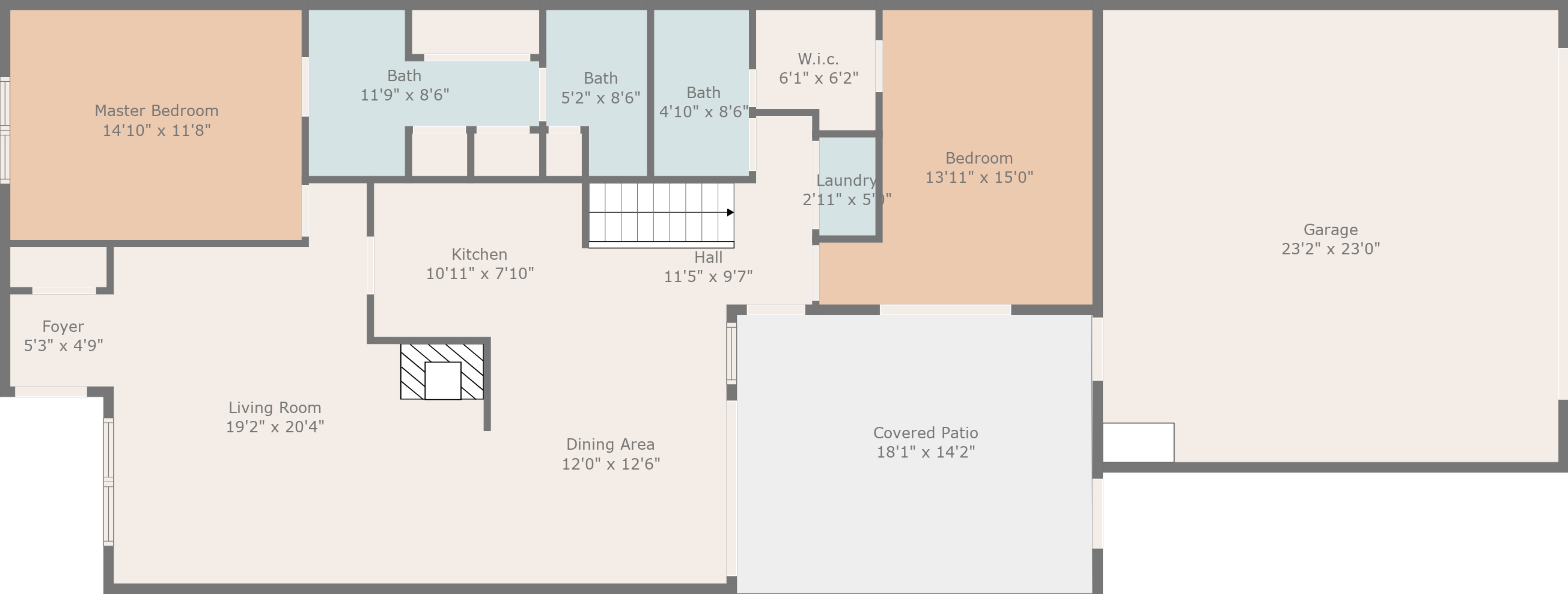
Floor 2
